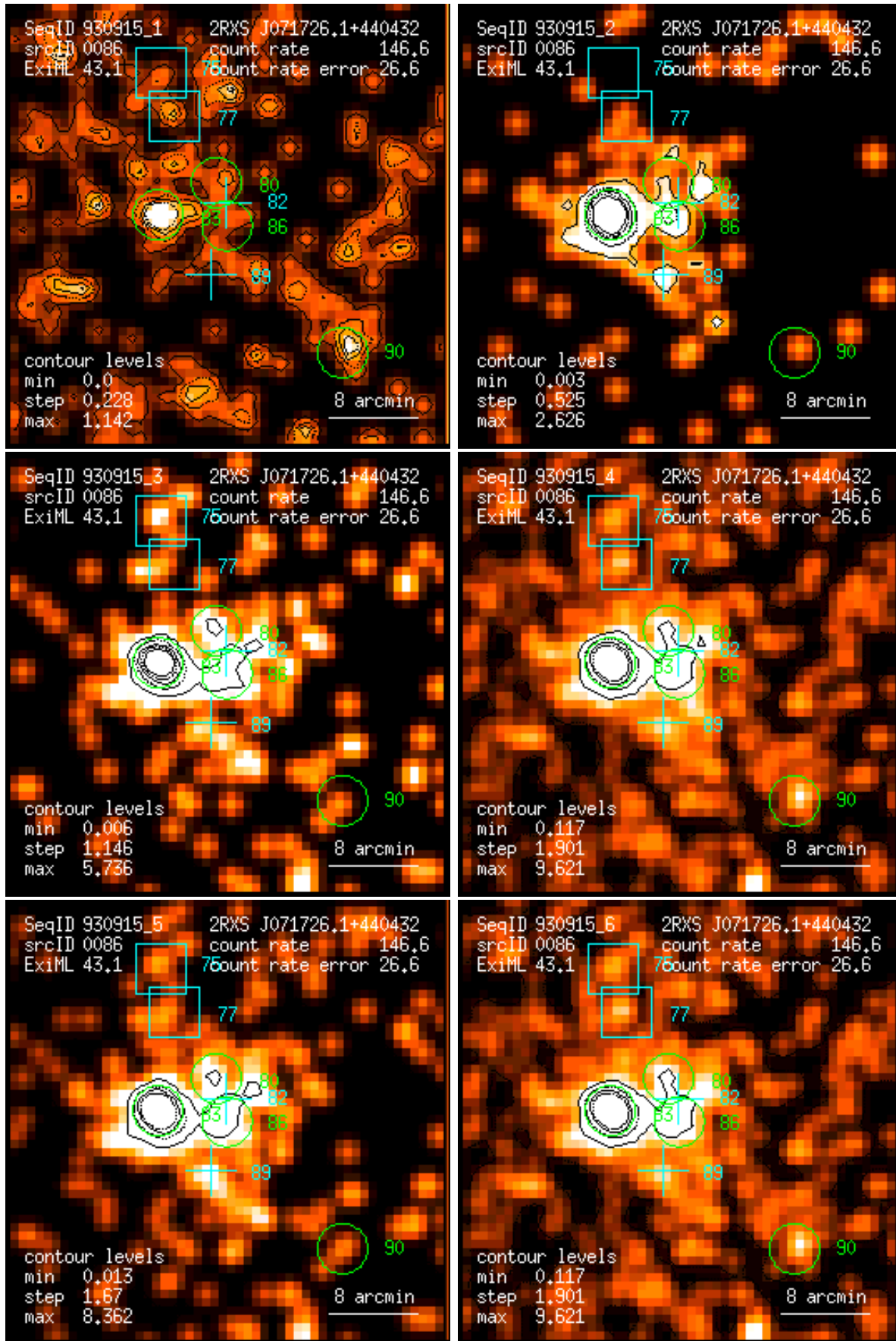
Figure 86: RASS 930915: detection 0086: band rate images, Gaussian filter: (1) PSPC channels 11 – 41, (2) 52 – 90, (3) 91 – 201, (4) 11 – 235, (5) 52 – 201, (6) 11 – 201. Broad band rates in counts/ks. Band rate contour levels in counts/ks/arcmin 2 .
