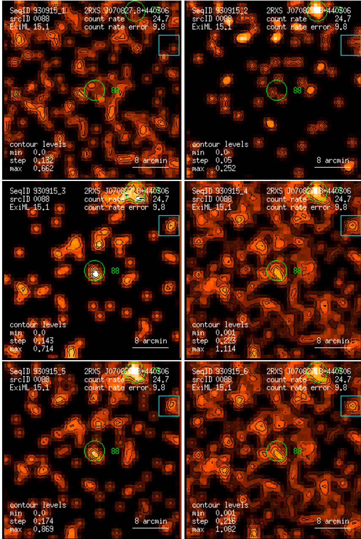
Figure 88: RASS 930915: detection 0088: band rate images, Gaussian filter: (1) PSPC channels 11 – 41, (2) 52 – 90, (3) 91 – 201, (4) 11 – 235, (5) 52 – 201, (6) 11 – 201. Broad band rates in counts/ks. Band rate contour levels in counts/ks/arcmin 2 .
