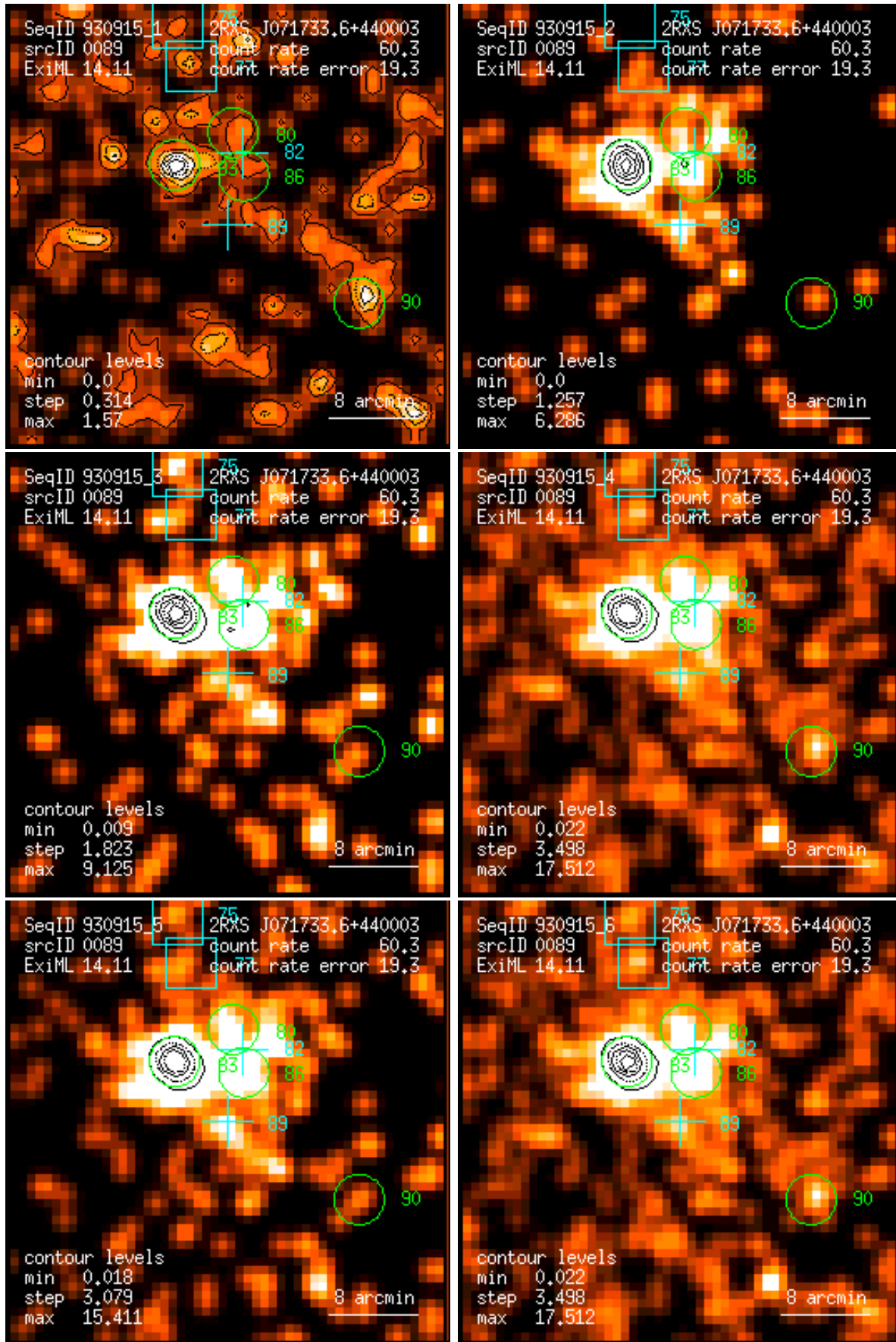
Figure 89: RASS 930915: detection 0089: band rate images, Gaussian filter: (1) PSPC channels 11 – 41, (2) 52 – 90, (3) 91 – 201, (4) 11 – 235, (5) 52 – 201, (6) 11 – 201. Broad band rates in counts/ks. Band rate contour levels in counts/ks/arcmin 2 .
