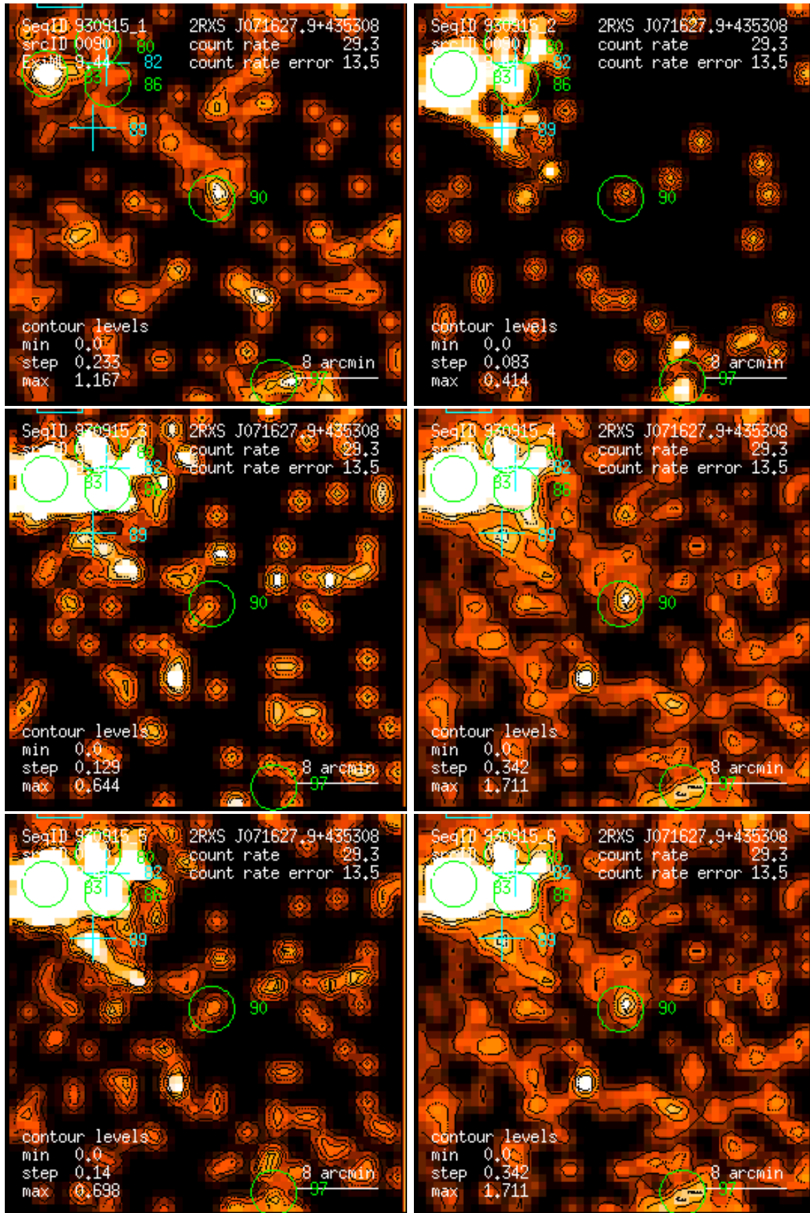
Figure 90: RASS 930915: detection 0090: band rate images, Gaussian filter: (1) PSPC channels 11 – 41, (2) 52 – 90, (3) 91 – 201, (4) 11 – 235, (5) 52 – 201, (6) 11 – 201. Broad band rates in counts/ks. Band rate contour levels in counts/ks/arcmin 2 .
