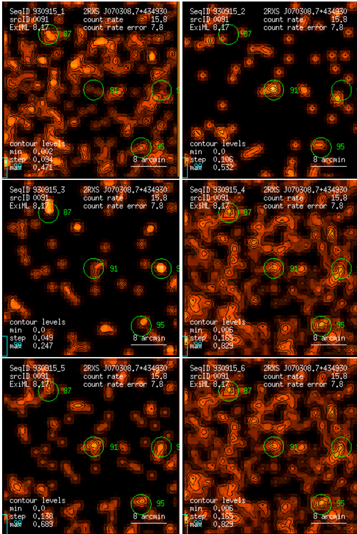
Figure 91: RASS 930915: detection 0091: band rate images, Gaussian filter: (1) PSPC channels 11 – 41, (2) 52 – 90, (3) 91 – 201, (4) 11 – 235, (5) 52 – 201, (6) 11 – 201. Broad band rates in counts/ks. Band rate contour levels in counts/ks/arcmin 2 .
