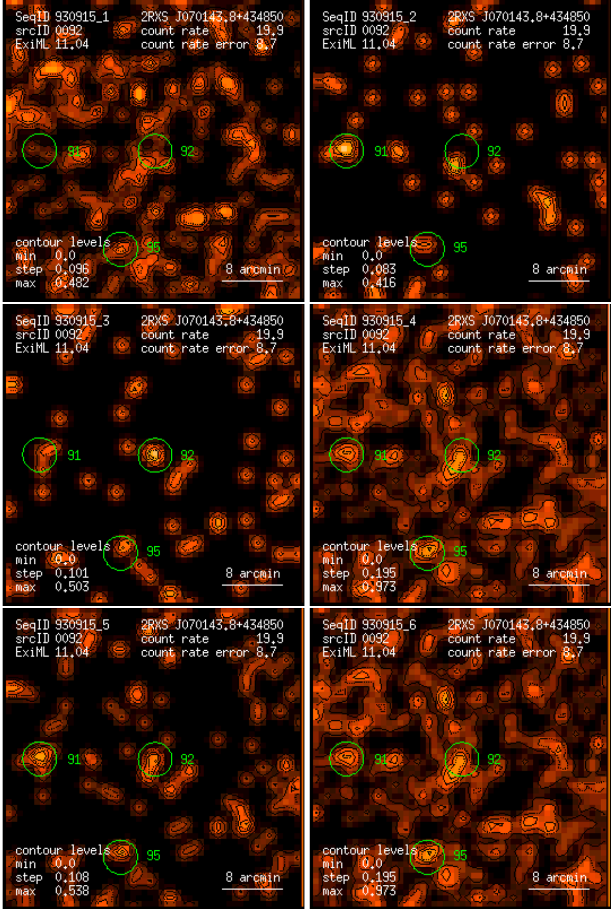
Figure 92: RASS 930915: detection 0092: band rate images, Gaussian filter: (1) PSPC channels 11 – 41, (2) 52 – 90, (3) 91 – 201, (4) 11 – 235, (5) 52 – 201, (6) 11 – 201. Broad band rates in counts/ks. Band rate contour levels in counts/ks/arcmin 2 .
