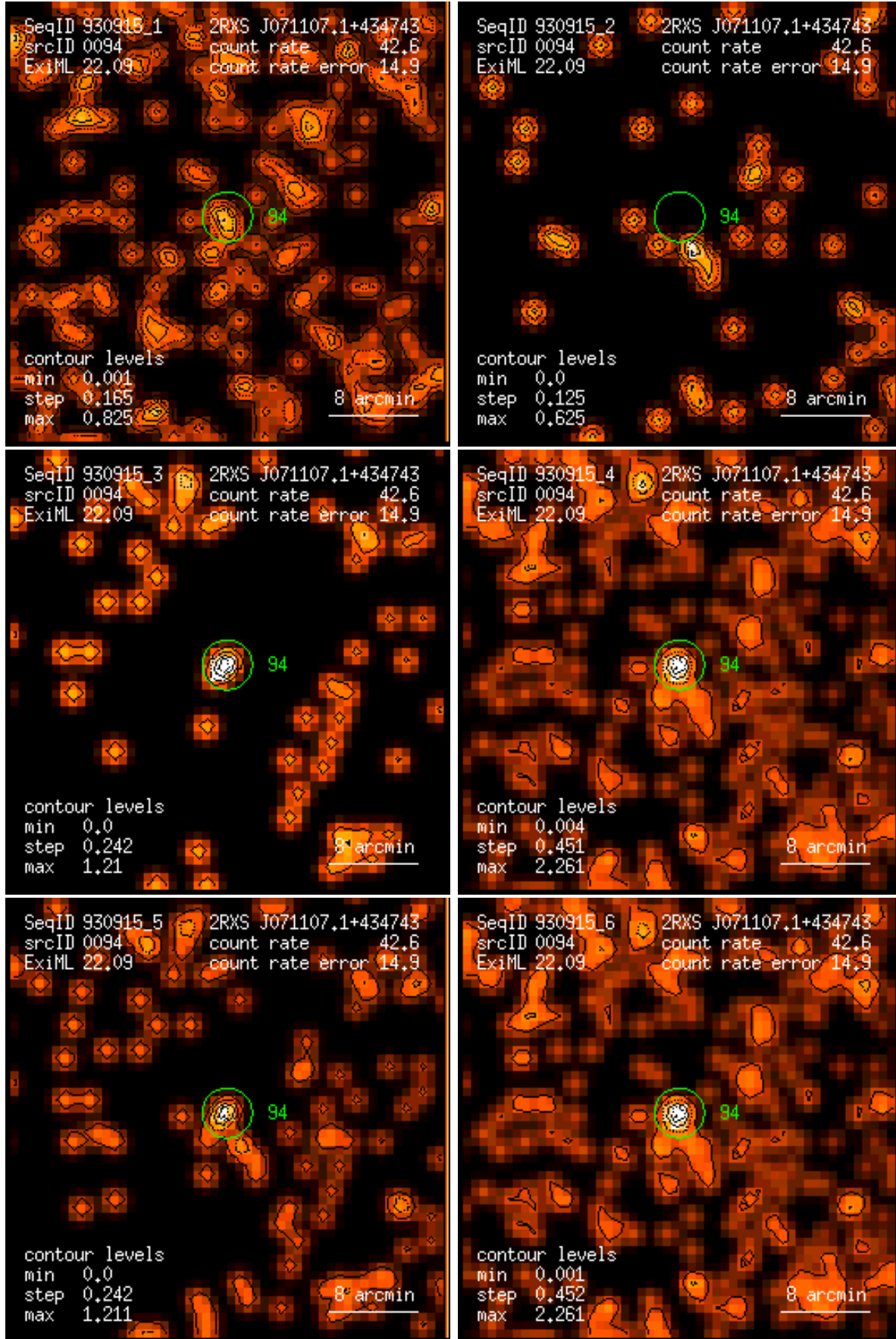
Figure 94: RASS 930915: detection 0094: band rate images, Gaussian filter: (1) PSPC channels 11 – 41, (2) 52 – 90, (3) 91 – 201, (4) 11 – 235, (5) 52 – 201, (6) 11 – 201. Broad band rates in counts/ks. Band rate contour levels in counts/ks/arcmin 2 .
