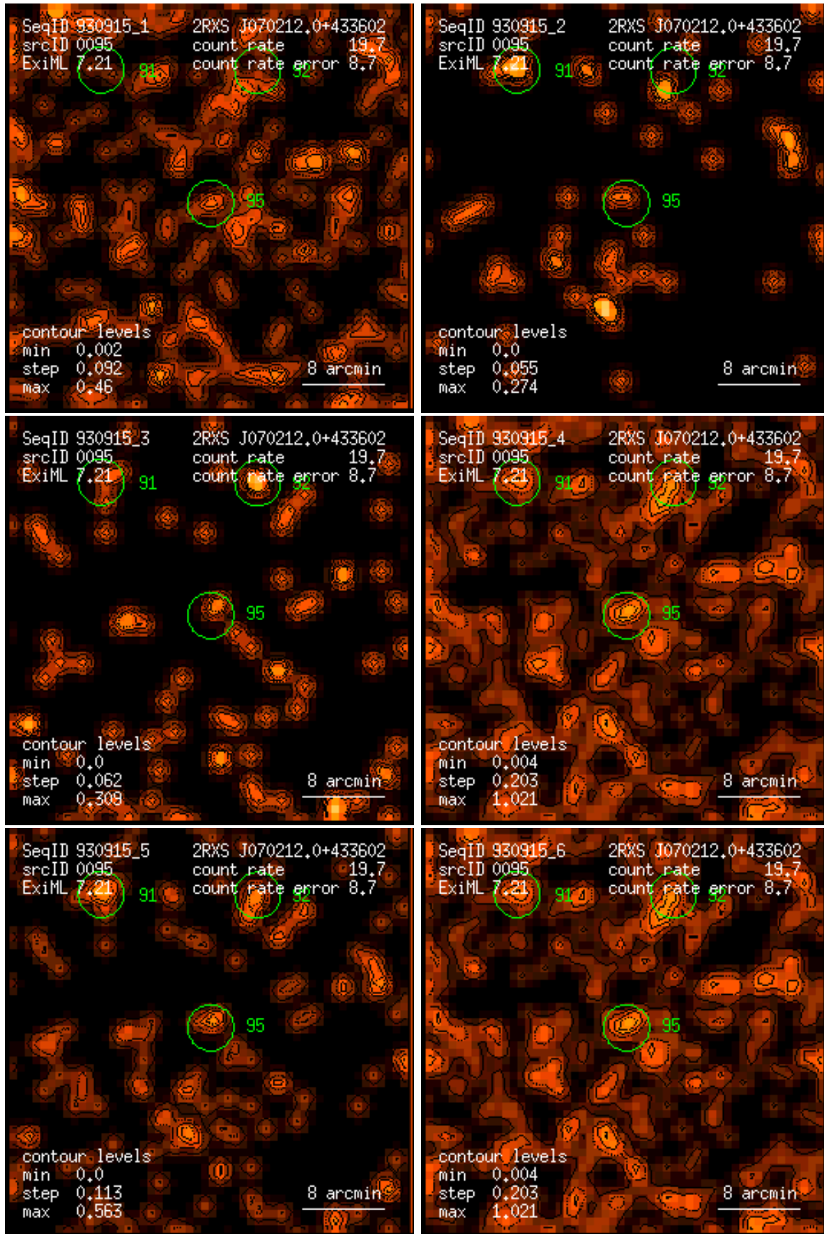
Figure 95: RASS 930915: detection 0095: band rate images, Gaussian filter: (1) PSPC channels 11 – 41, (2) 52 – 90, (3) 91 – 201, (4) 11 – 235, (5) 52 – 201, (6) 11 – 201. Broad band rates in counts/ks. Band rate contour levels in counts/ks/arcmin 2 .
