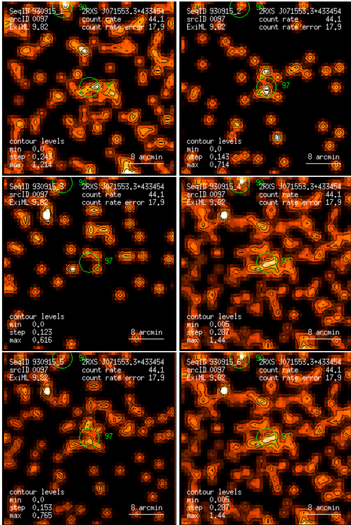
Figure 97: RASS 930915: detection 0097: band rate images, Gaussian filter: (1) PSPC channels 11 – 41, (2) 52 – 90, (3) 91 – 201, (4) 11 – 235, (5) 52 – 201, (6) 11 – 201. Broad band rates in counts/ks. Band rate contour levels in counts/ks/arcmin 2 .
