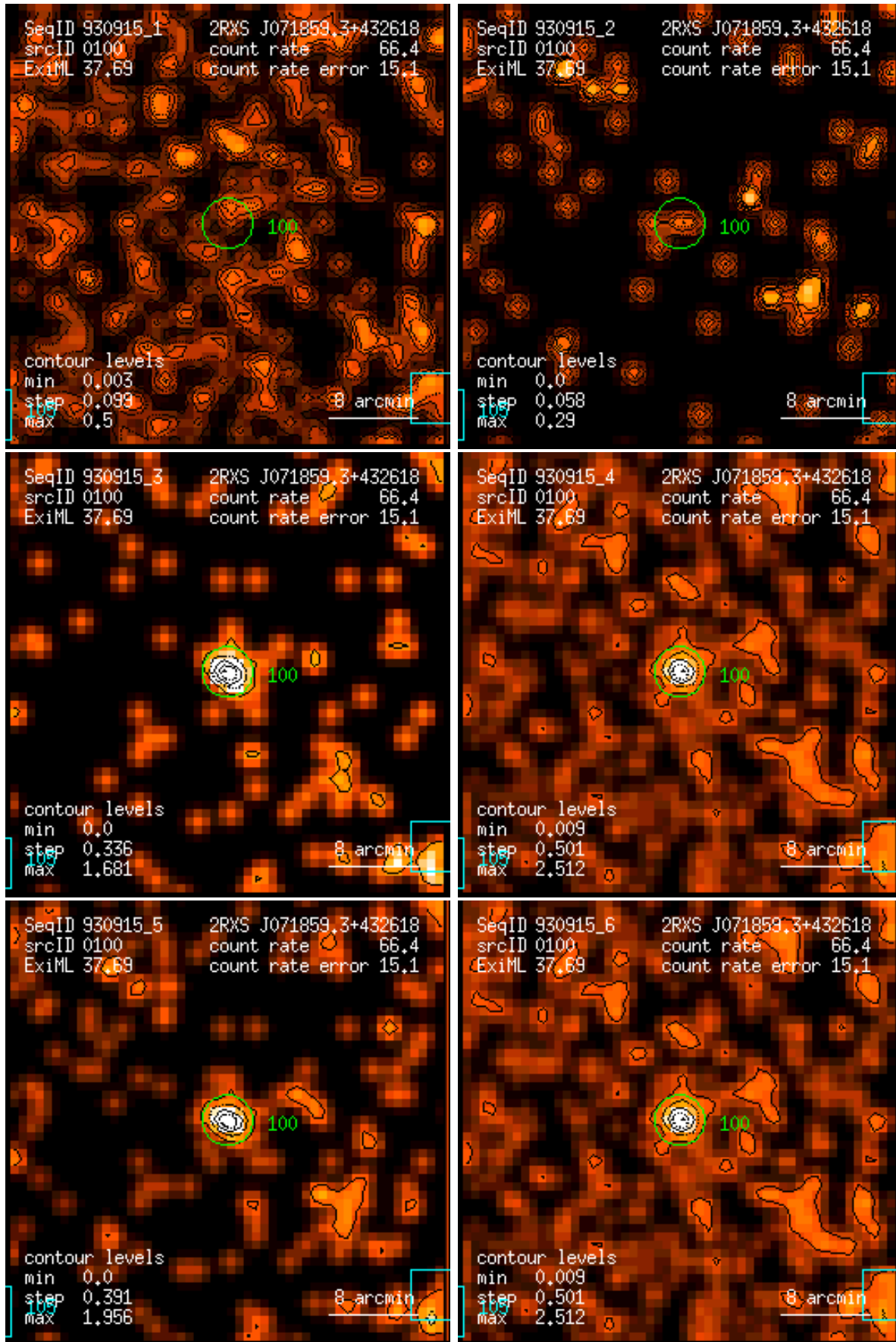
Figure 100: RASS 930915: detection 0100: band rate images, Gaussian filter: (1) PSPC channels 11 – 41, (2) 52 – 90, (3) 91 – 201, (4) 11 – 235, (5) 52 – 201, (6) 11 – 201. Broad band rates in counts/ks. Band rate contour levels in counts/ks/arcmin 2 .
