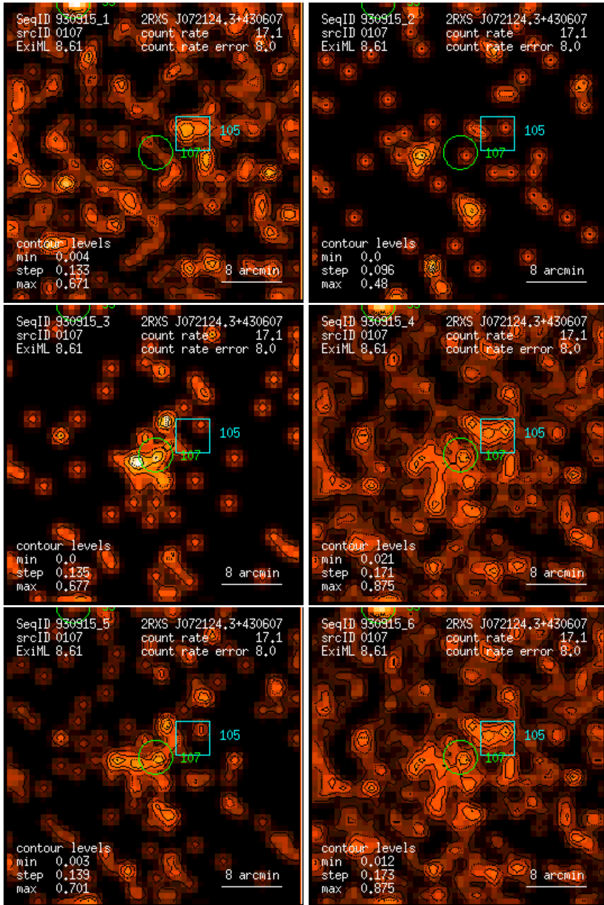
Figure 107: RASS 930915: detection 0107: band rate images, Gaussian filter: (1) PSPC channels 11 – 41, (2) 52 – 90, (3) 91 – 201, (4) 11 – 235, (5) 52 – 201, (6) 11 – 201. Broad band rates in counts/ks. Band rate contour levels in counts/ks/arcmin 2 .
