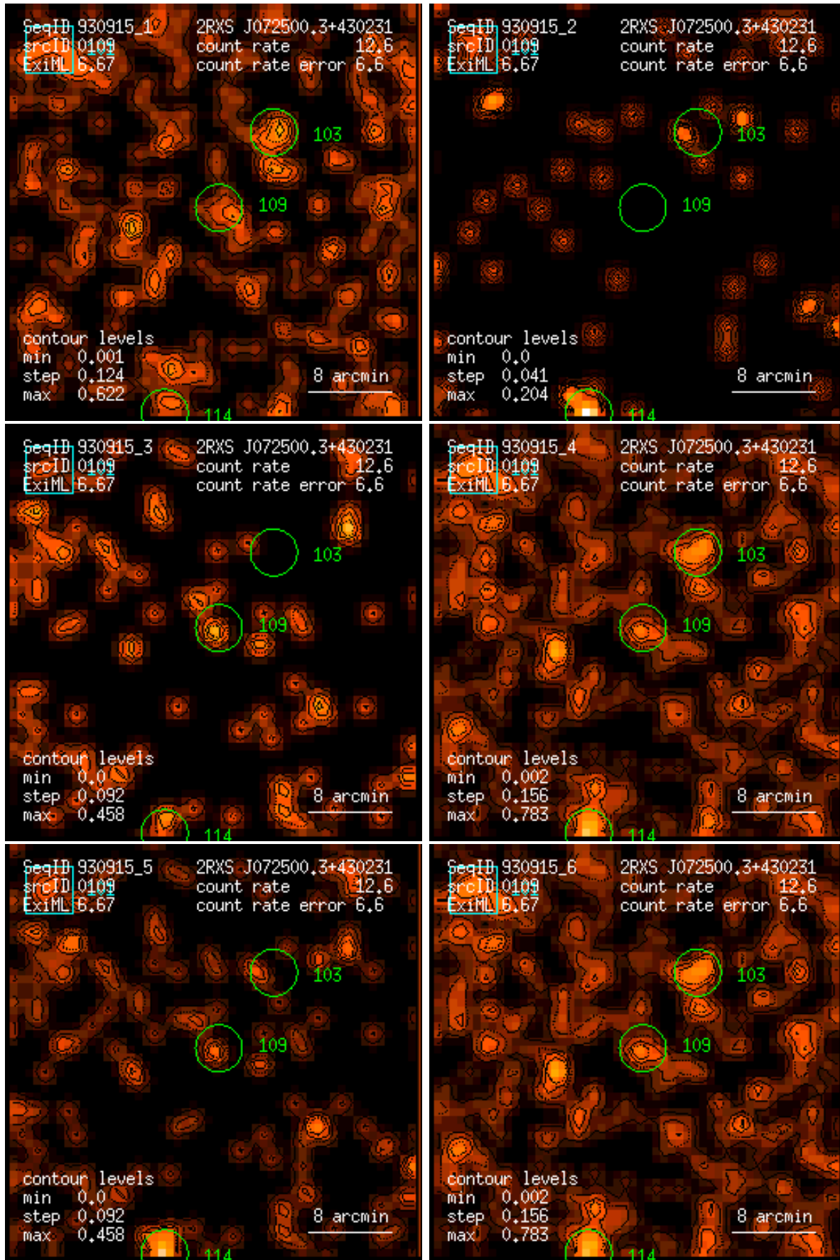
Figure 109: RASS 930915: detection 0109: band rate images, Gaussian filter: (1) PSPC channels 11 – 41, (2) 52 – 90, (3) 91 – 201, (4) 11 – 235, (5) 52 – 201, (6) 11 – 201. Broad band rates in counts/ks. Band rate contour levels in counts/ks/arcmin 2 .
