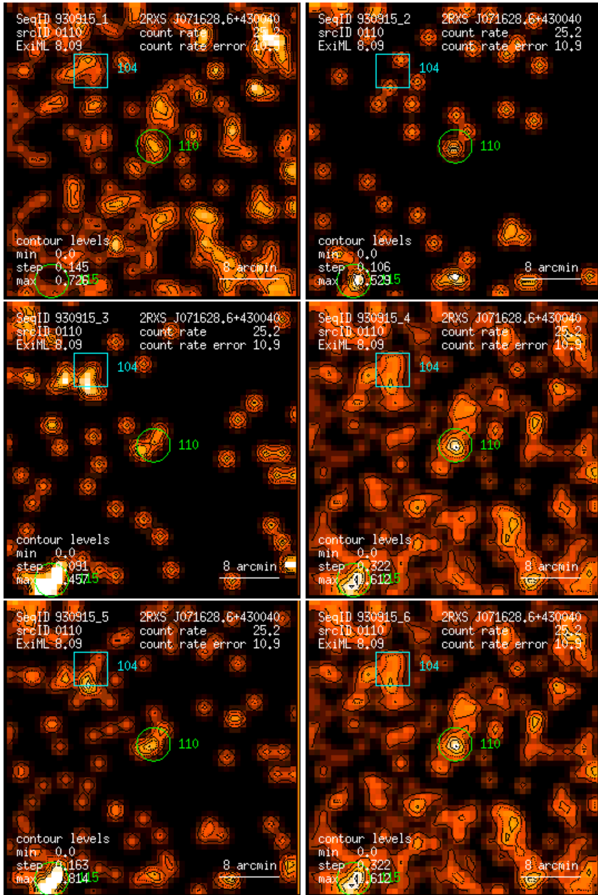
Figure 110: RASS 930915: detection 0110: band rate images, Gaussian filter: (1) PSPC channels 11 – 41, (2) 52 – 90, (3) 91 – 201, (4) 11 – 235, (5) 52 – 201, (6) 11 – 201. Broad band rates in counts/ks. Band rate contour levels in counts/ks/arcmin 2 .
