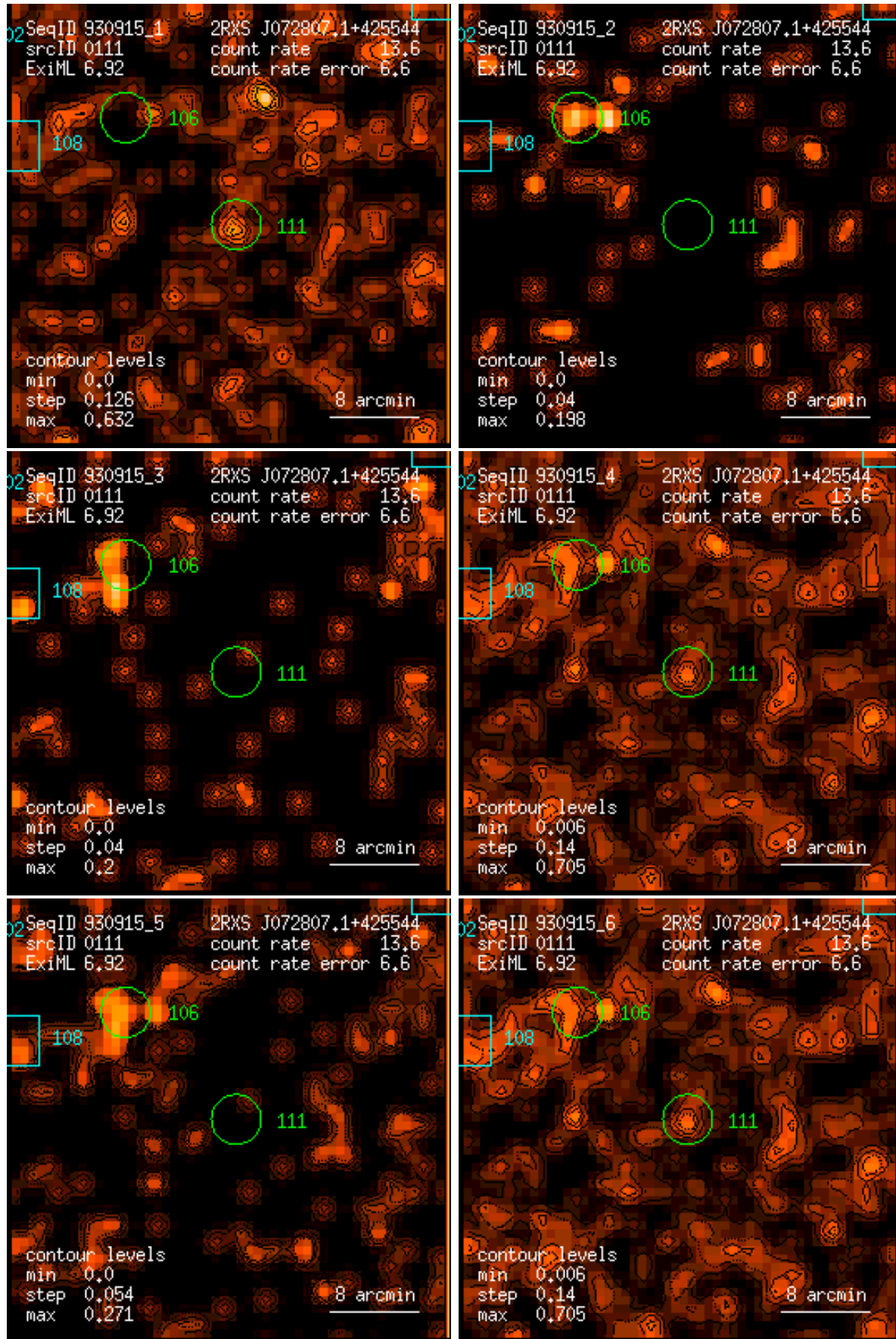
Figure 111: RASS 930915: detection 0111: band rate images, Gaussian filter: (1) PSPC channels 11 – 41, (2) 52 – 90, (3) 91 – 201, (4) 11 – 235, (5) 52 – 201, (6) 11 – 201. Broad band rates in counts/ks. Band rate contour levels in counts/ks/arcmin 2 .
