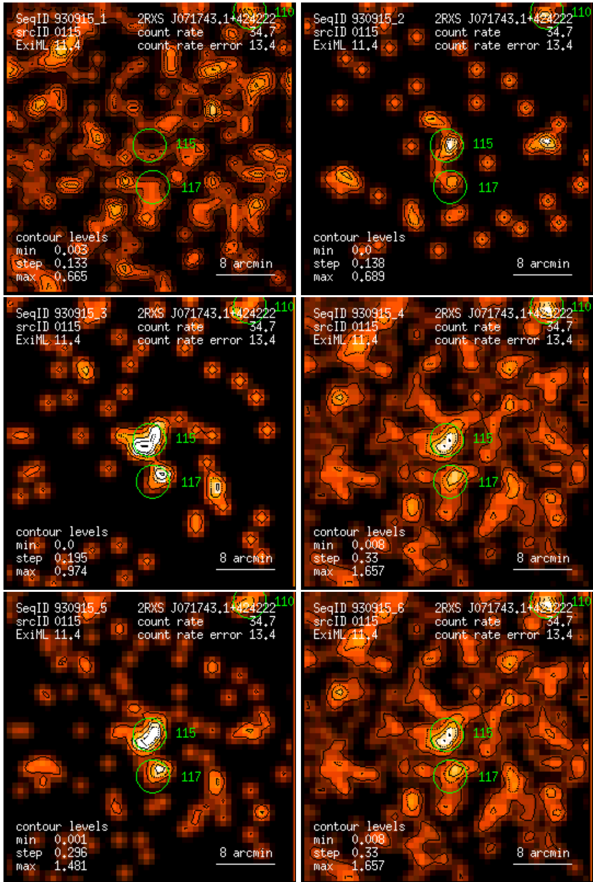
Figure 115: RASS 930915: detection 0115: band rate images, Gaussian filter: (1) PSPC channels 11 – 41, (2) 52 – 90, (3) 91 – 201, (4) 11 – 235, (5) 52 – 201, (6) 11 – 201. Broad band rates in counts/ks. Band rate contour levels in counts/ks/arcmin 2 .
