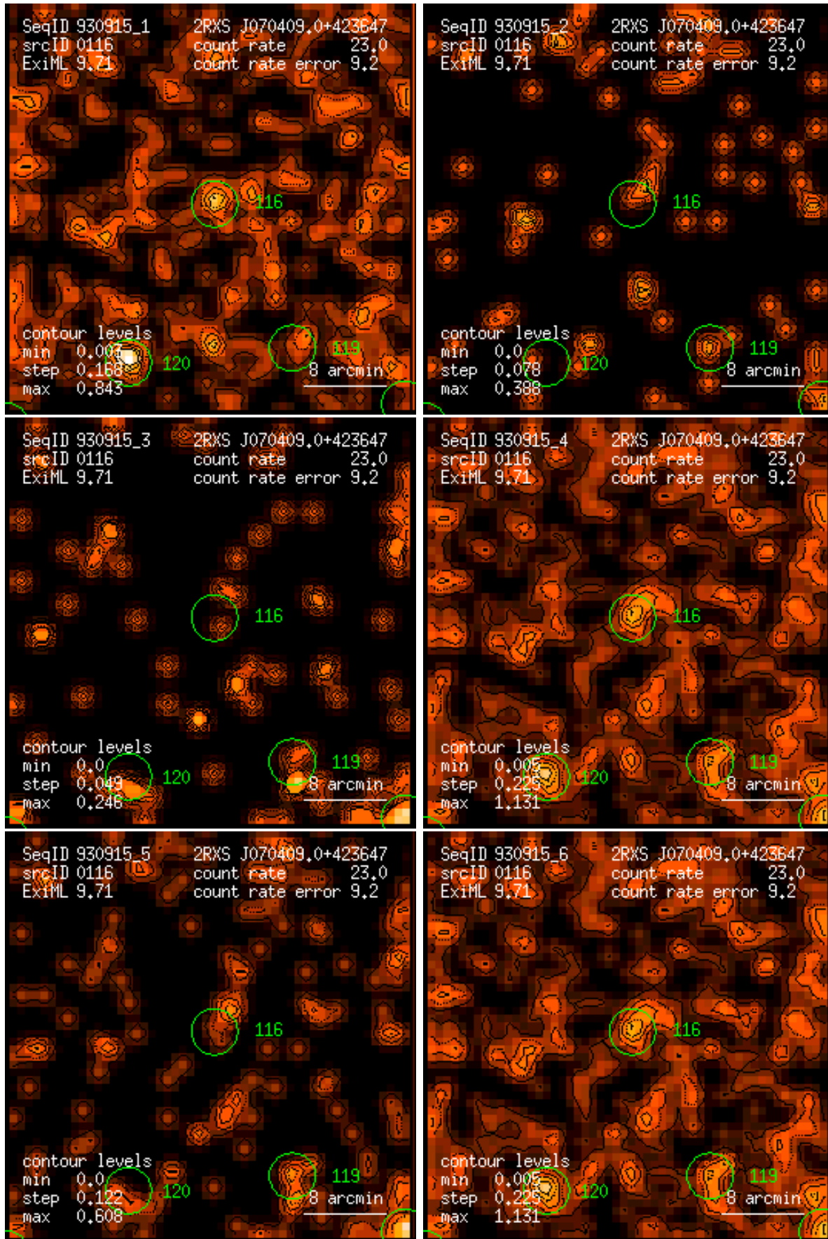
Figure 116: RASS 930915: detection 0116: band rate images, Gaussian filter: (1) PSPC channels 11 – 41, (2) 52 – 90, (3) 91 – 201, (4) 11 – 235, (5) 52 – 201, (6) 11 – 201. Broad band rates in counts/ks. Band rate contour levels in counts/ks/arcmin 2 .
