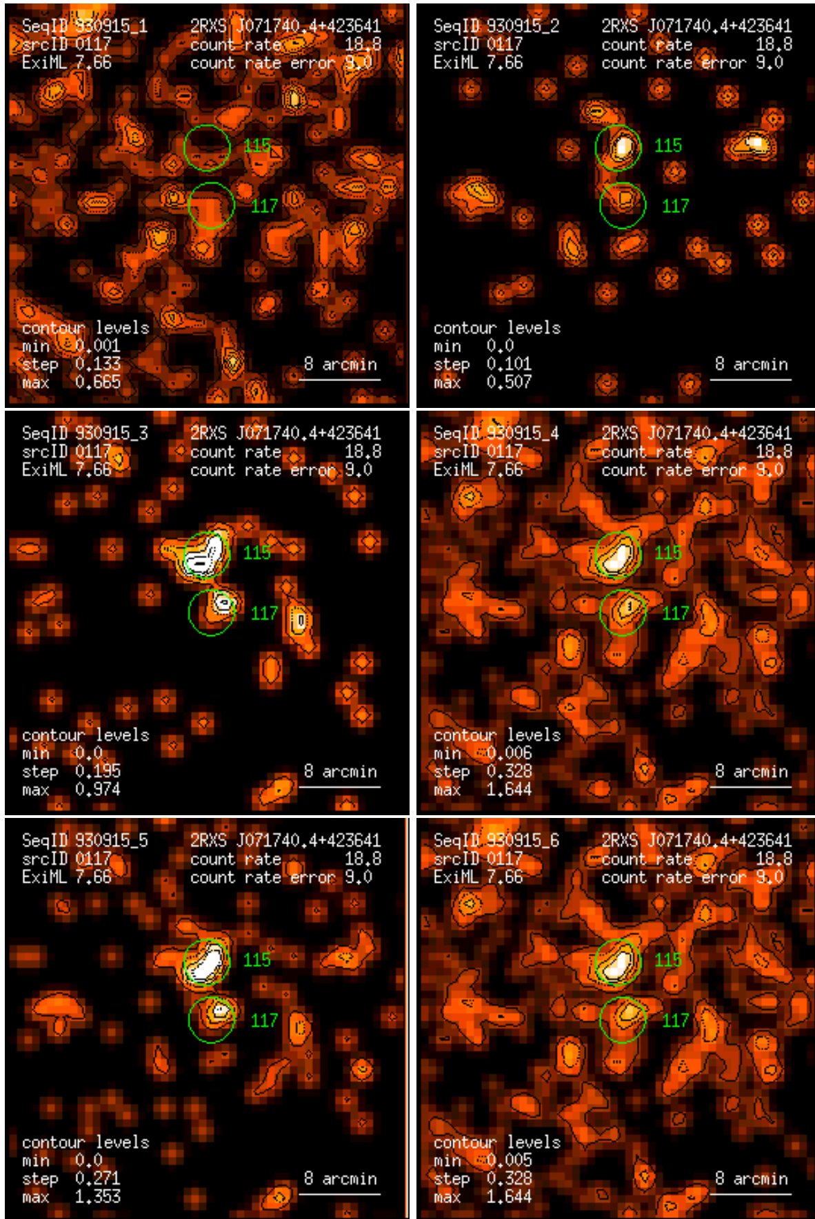
Figure 117: RASS 930915: detection 0117: band rate images, Gaussian filter: (1) PSPC channels 11 – 41, (2) 52 – 90, (3) 91 – 201, (4) 11 – 235, (5) 52 – 201, (6) 11 – 201. Broad band rates in counts/ks. Band rate contour levels in counts/ks/arcmin 2 .
