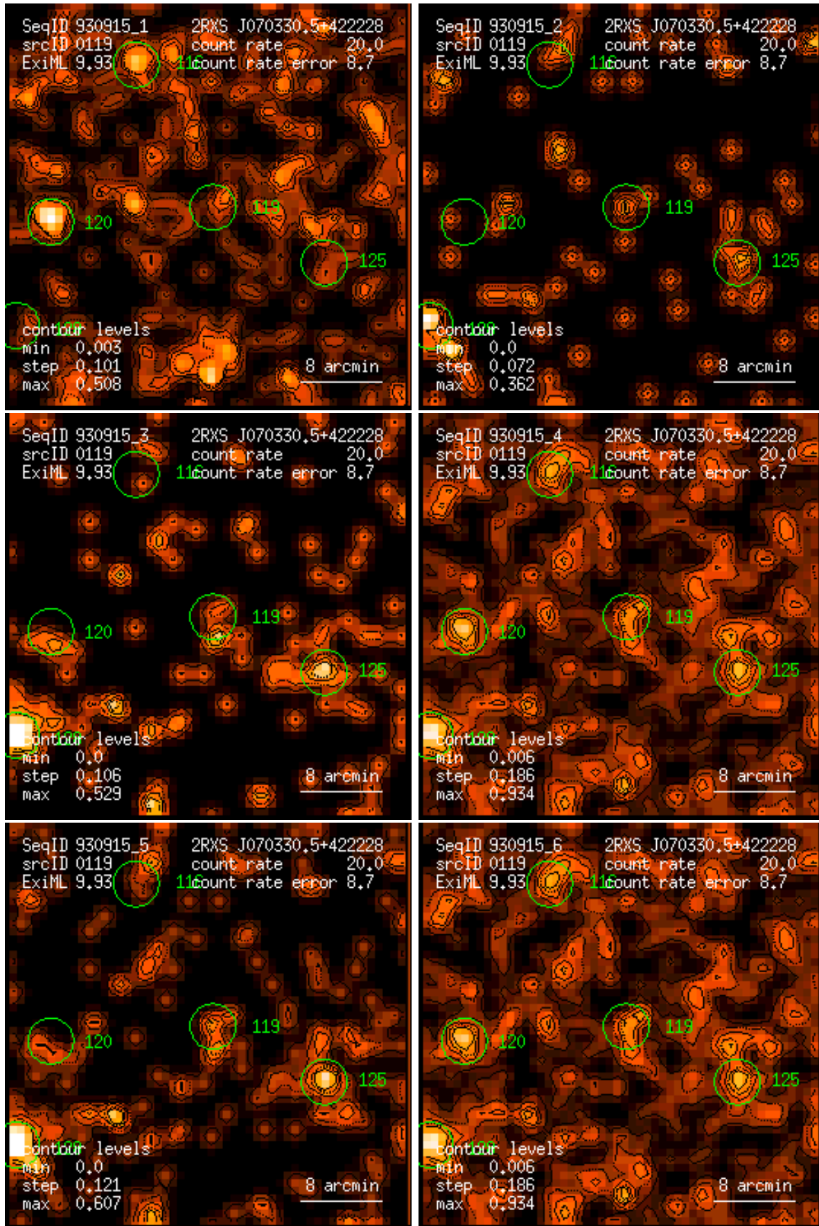
Figure 119: RASS 930915: detection 0119: band rate images, Gaussian filter: (1) PSPC channels 11 – 41, (2) 52 – 90, (3) 91 – 201, (4) 11 – 235, (5) 52 – 201, (6) 11 – 201. Broad band rates in counts/ks. Band rate contour levels in counts/ks/arcmin 2 .
