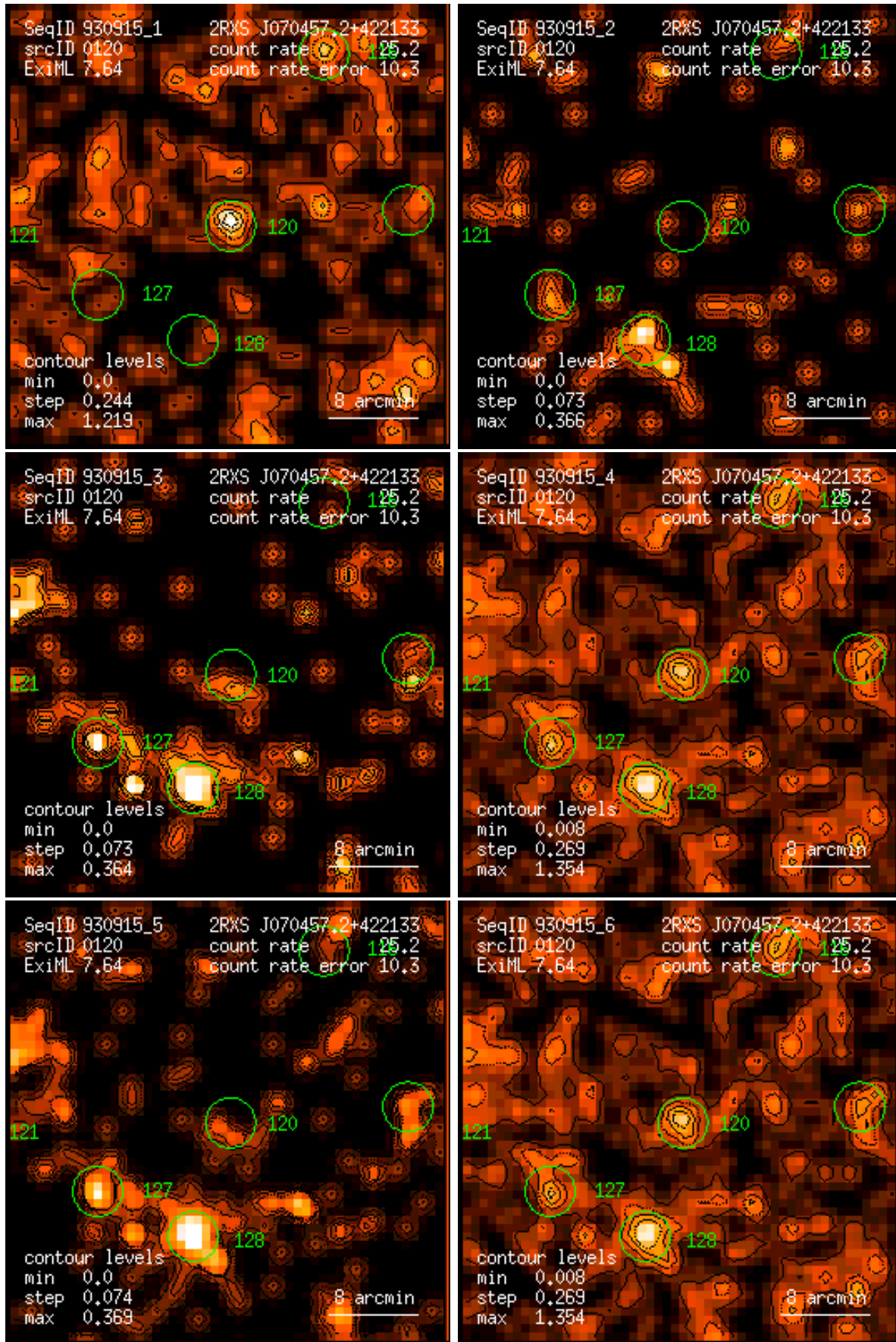
Figure 120: RASS 930915: detection 0120: band rate images, Gaussian filter: (1) PSPC channels 11 – 41, (2) 52 – 90, (3) 91 – 201, (4) 11 – 235, (5) 52 – 201, (6) 11 – 201. Broad band rates in counts/ks. Band rate contour levels in counts/ks/arcmin 2 .
