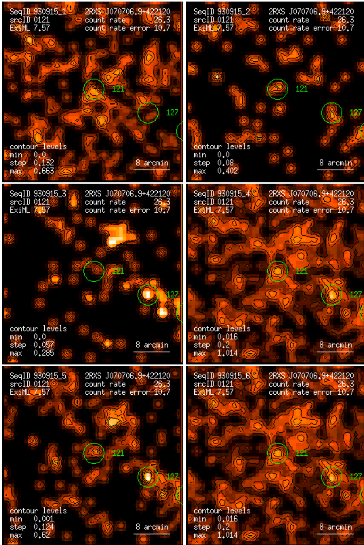
Figure 121: RASS 930915: detection 0121: band rate images, Gaussian filter: (1) PSPC channels 11 – 41, (2) 52 – 90, (3) 91 – 201, (4) 11 – 235, (5) 52 – 201, (6) 11 – 201. Broad band rates in counts/ks. Band rate contour levels in counts/ks/arcmin 2 .
