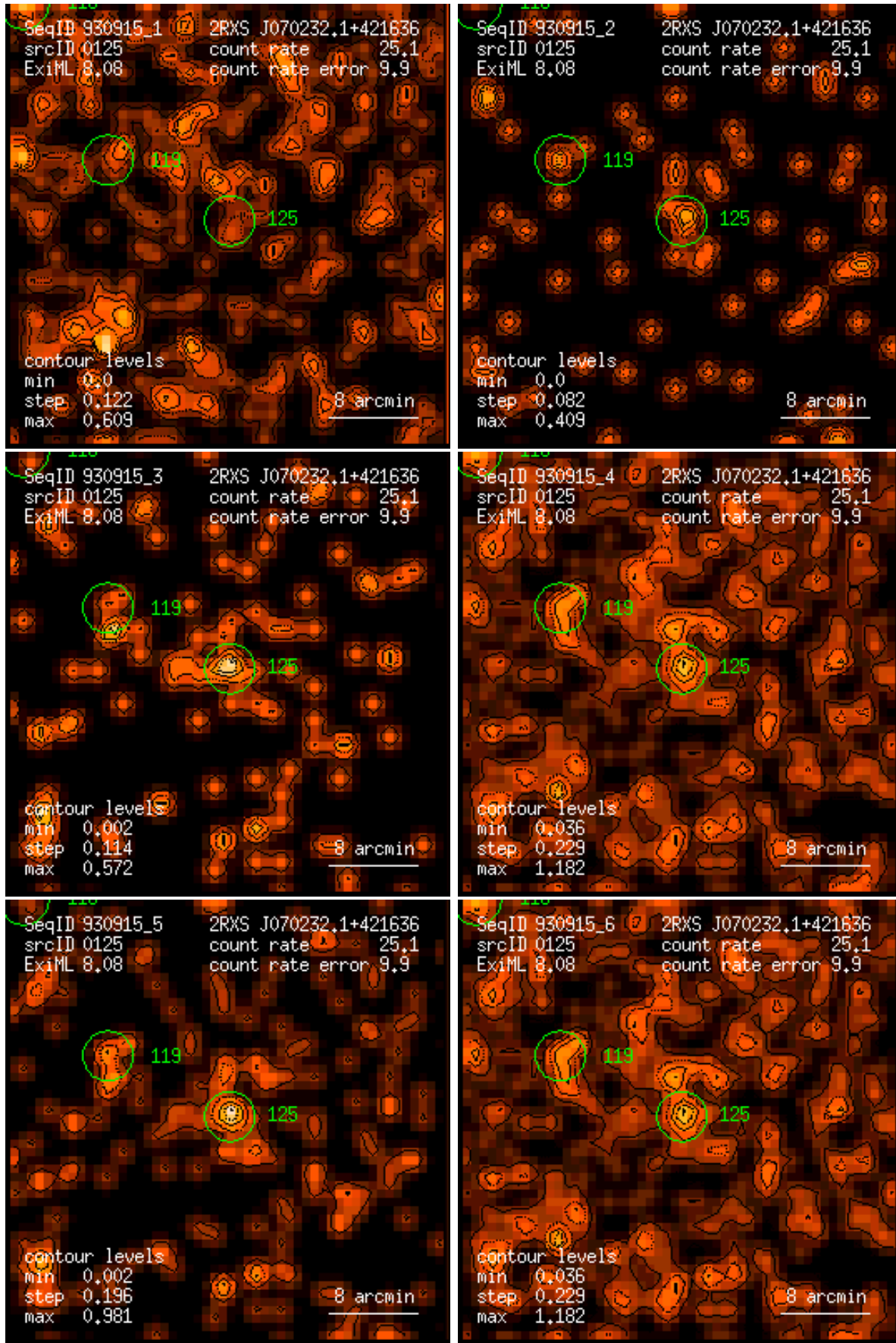
Figure 125: RASS 930915: detection 0125: band rate images, Gaussian filter: (1) PSPC channels 11 – 41, (2) 52 – 90, (3) 91 – 201, (4) 11 – 235, (5) 52 – 201, (6) 11 – 201. Broad band rates in counts/ks. Band rate contour levels in counts/ks/arcmin 2 .
