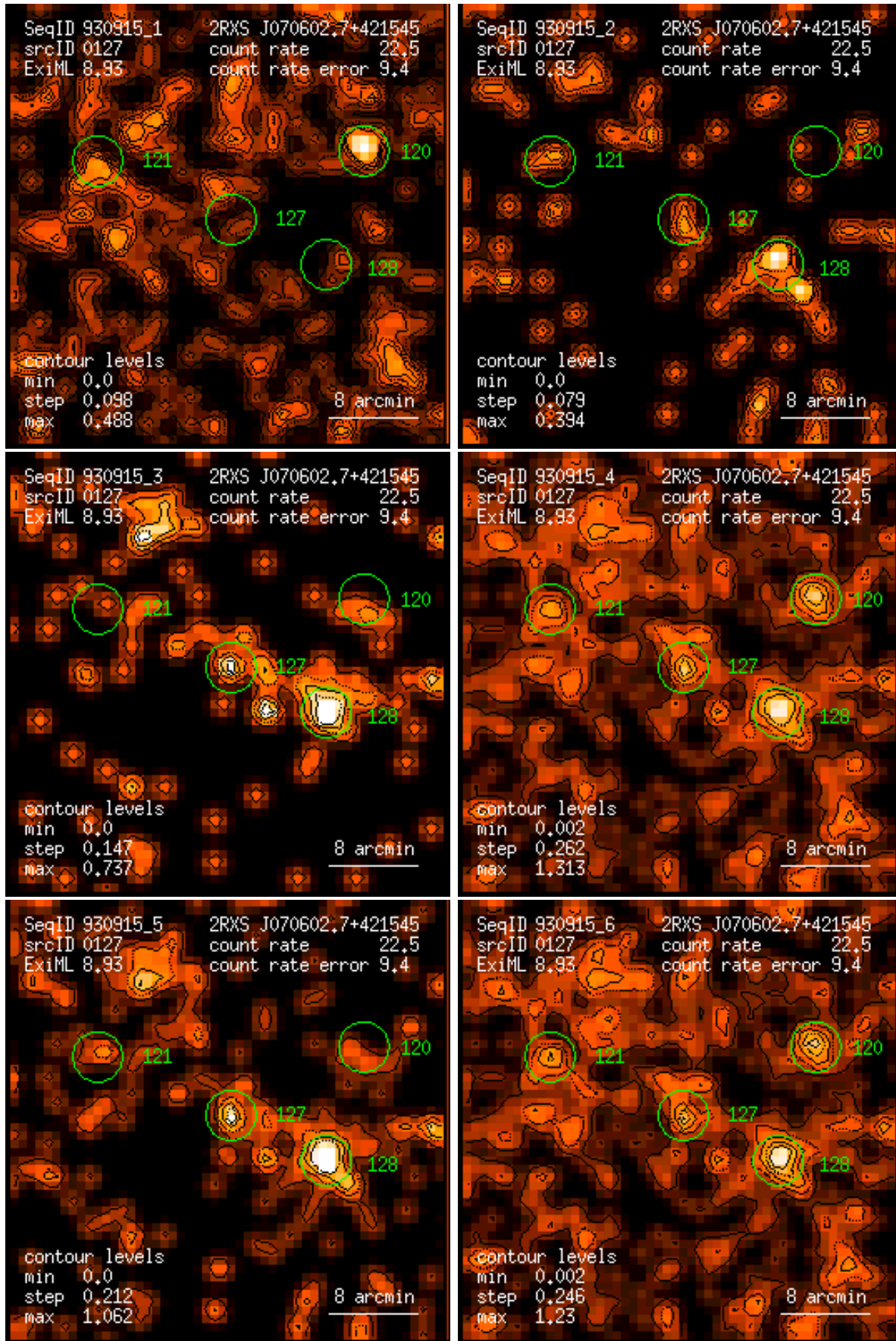
Figure 127: RASS 930915: detection 0127: band rate images, Gaussian filter: (1) PSPC channels 11 – 41, (2) 52 – 90, (3) 91 – 201, (4) 11 – 235, (5) 52 – 201, (6) 11 – 201. Broad band rates in counts/ks. Band rate contour levels in counts/ks/arcmin 2 .
