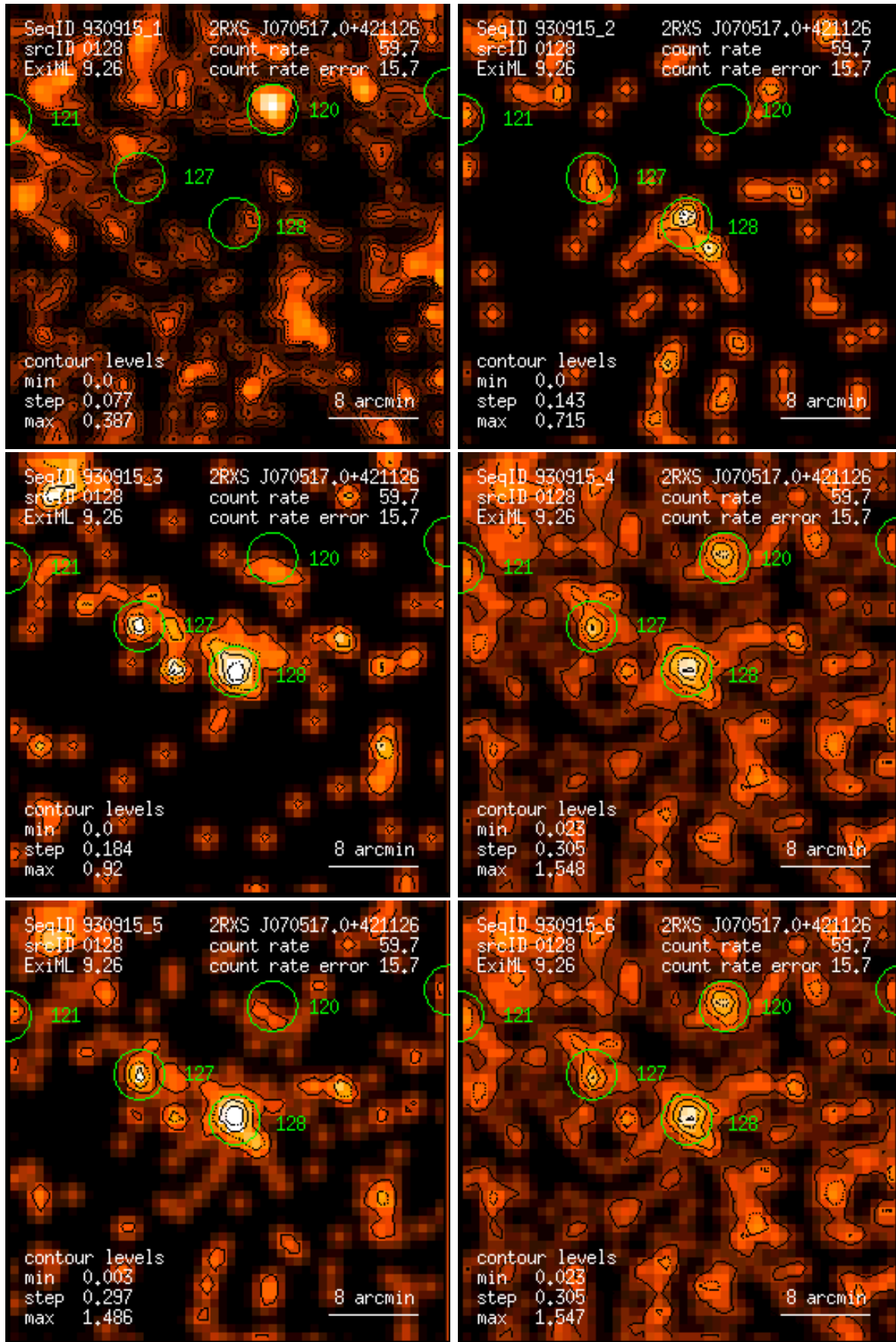
Figure 128: RASS 930915: detection 0128: band rate images, Gaussian filter: (1) PSPC channels 11 – 41, (2) 52 – 90, (3) 91 – 201, (4) 11 – 235, (5) 52 – 201, (6) 11 – 201. Broad band rates in counts/ks. Band rate contour levels in counts/ks/arcmin 2 .
