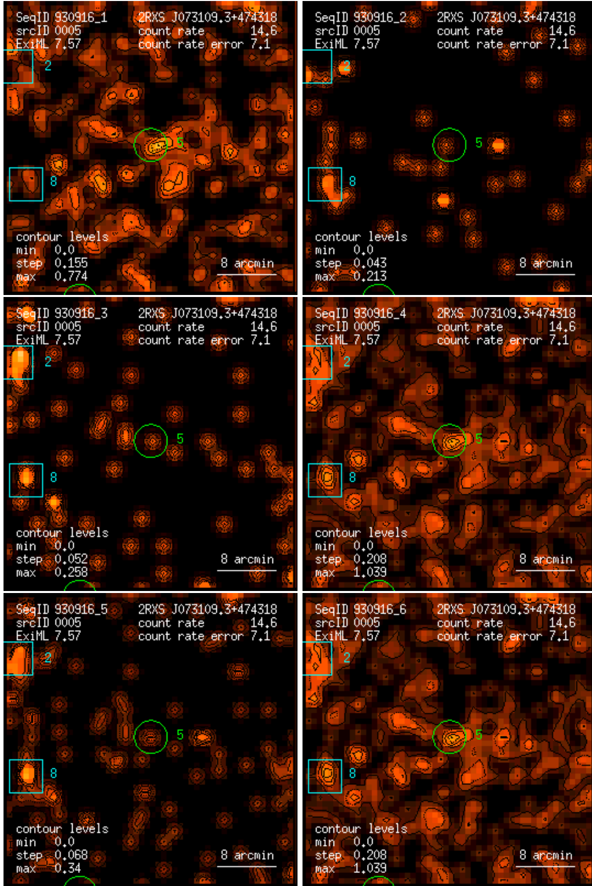
Figure 5: RASS 930916: detection 0005: band rate images, Gaussian filter: (1) PSPC channels 11 – 41, (2) 52 – 90, (3) 91 – 201, (4) 11 – 235, (5) 52 – 201, (6) 11 – 201. Broad band rates in counts/ks. Band rate contour levels in counts/ks/arcmin 2 .
