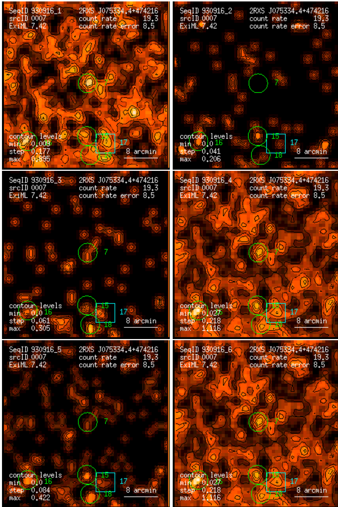
Figure 7: RASS 930916: detection 0007: band rate images, Gaussian filter: (1) PSPC channels 11 – 41, (2) 52 – 90, (3) 91 – 201, (4) 11 – 235, (5) 52 – 201, (6) 11 – 201. Broad band rates in counts/ks. Band rate contour levels in counts/ks/arcmin 2 .
