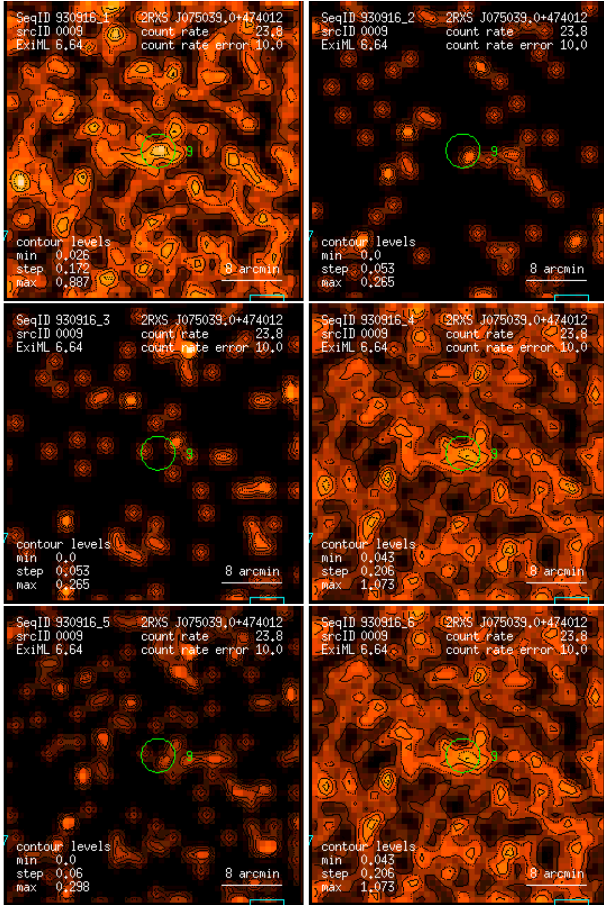
Figure 9: RASS 930916: detection 0009: band rate images, Gaussian filter: (1) PSPC channels 11 – 41, (2) 52 – 90, (3) 91 – 201, (4) 11 – 235, (5) 52 – 201, (6) 11 – 201. Broad band rates in counts/ks. Band rate contour levels in counts/ks/arcmin 2 .
