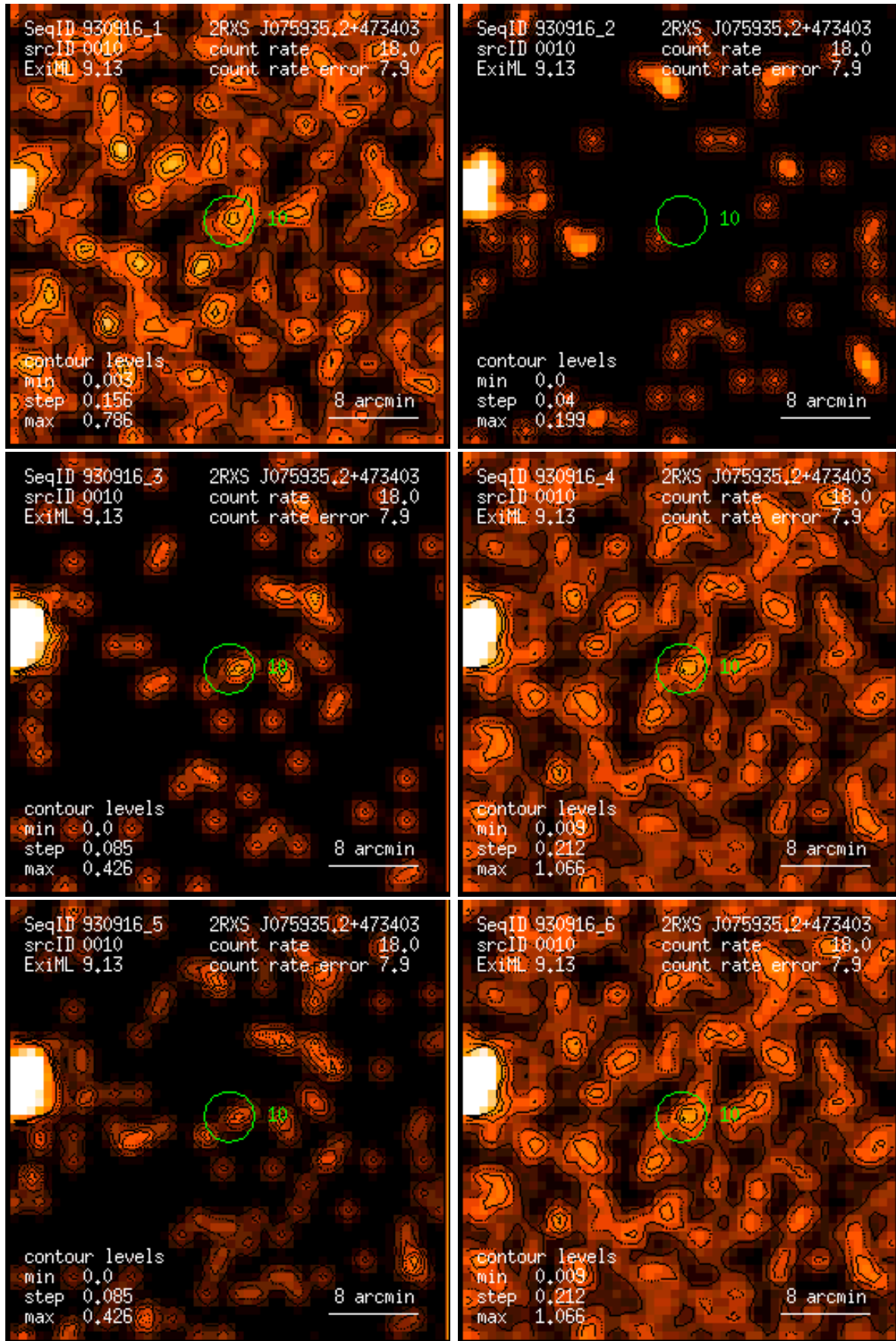
Figure 10: RASS 930916: detection 0010: band rate images, Gaussian filter: (1) PSPC channels 11 – 41, (2) 52 – 90, (3) 91 – 201, (4) 11 – 235, (5) 52 – 201, (6) 11 – 201. Broad band rates in counts/ks. Band rate contour levels in counts/ks/arcmin 2 .
