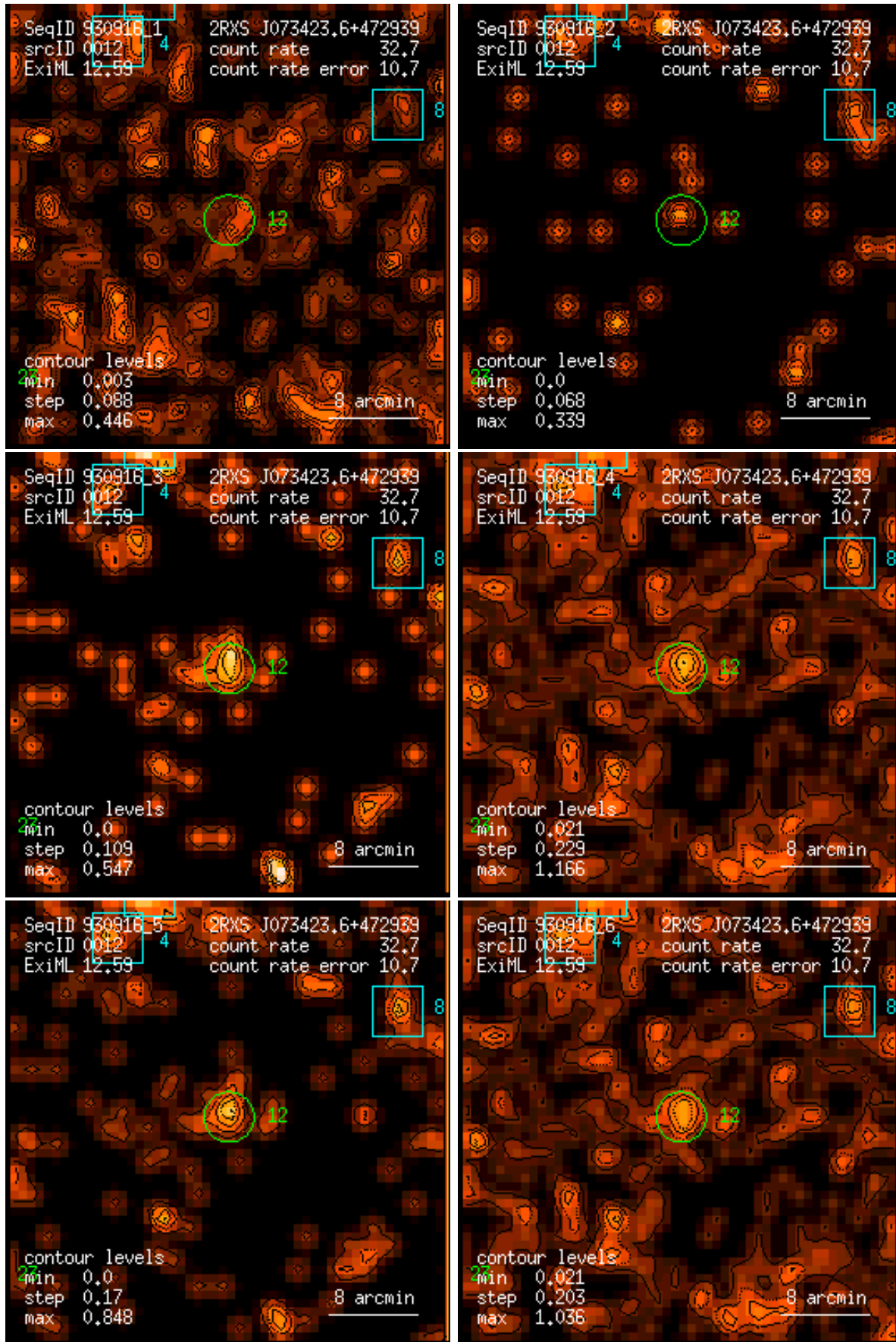
Figure 12: RASS 930916: detection 0012: band rate images, Gaussian filter: (1) PSPC channels 11 – 41, (2) 52 – 90, (3) 91 – 201, (4) 11 – 235, (5) 52 – 201, (6) 11 – 201. Broad band rates in counts/ks. Band rate contour levels in counts/ks/arcmin 2 .
