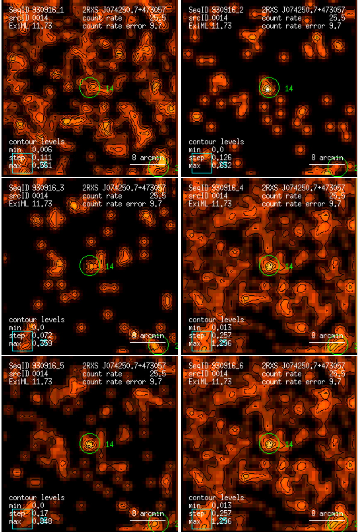
Figure 14: RASS 930916: detection 0014: band rate images, Gaussian filter: (1) PSPC channels 11 – 41, (2) 52 – 90, (3) 91 – 201, (4) 11 – 235, (5) 52 – 201, (6) 11 – 201. Broad band rates in counts/ks. Band rate contour levels in counts/ks/arcmin 2 .
