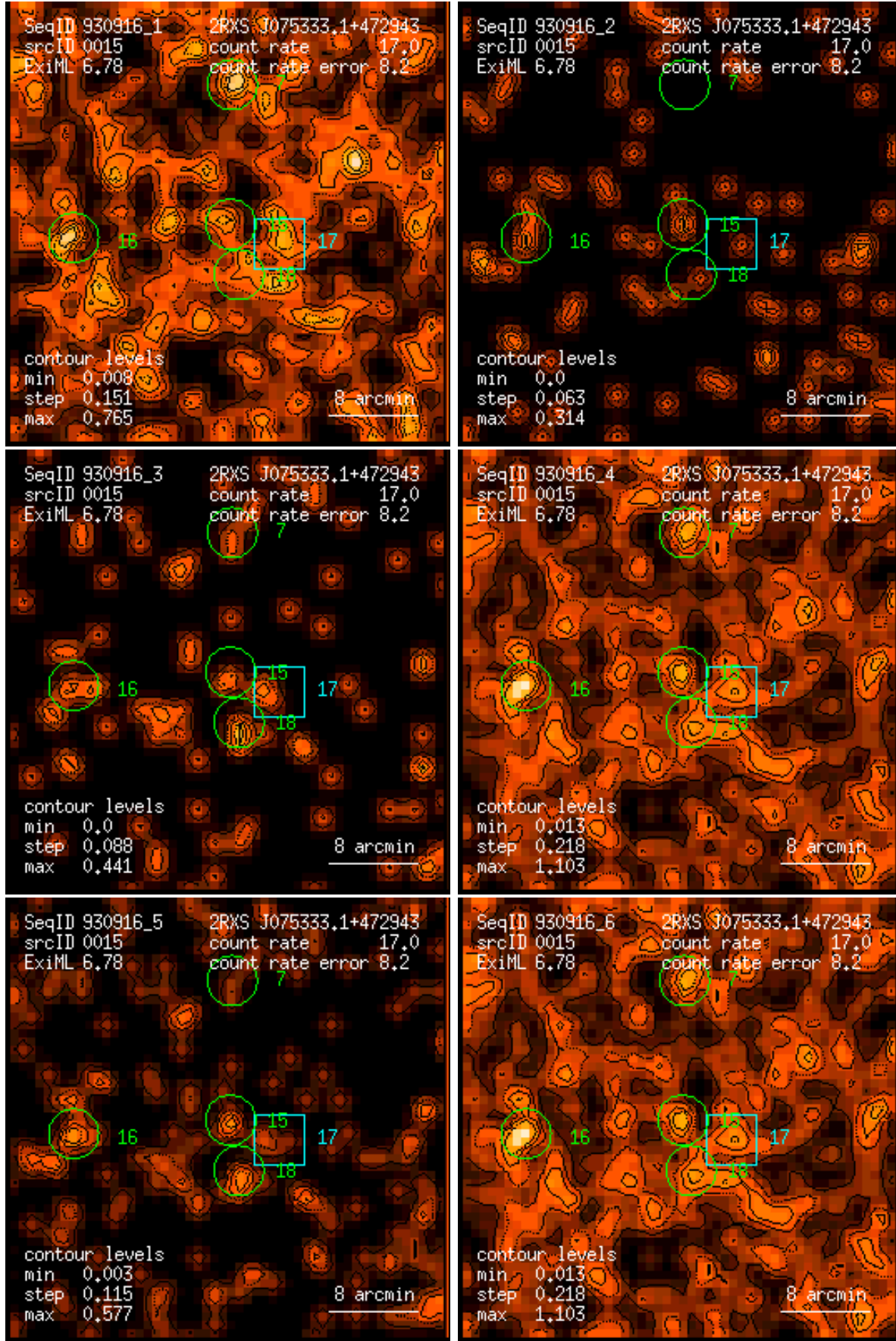
Figure 15: RASS 930916: detection 0015: band rate images, Gaussian filter: (1) PSPC channels 11 – 41, (2) 52 – 90, (3) 91 – 201, (4) 11 – 235, (5) 52 – 201, (6) 11 – 201. Broad band rates in counts/ks. Band rate contour levels in counts/ks/arcmin 2 .
