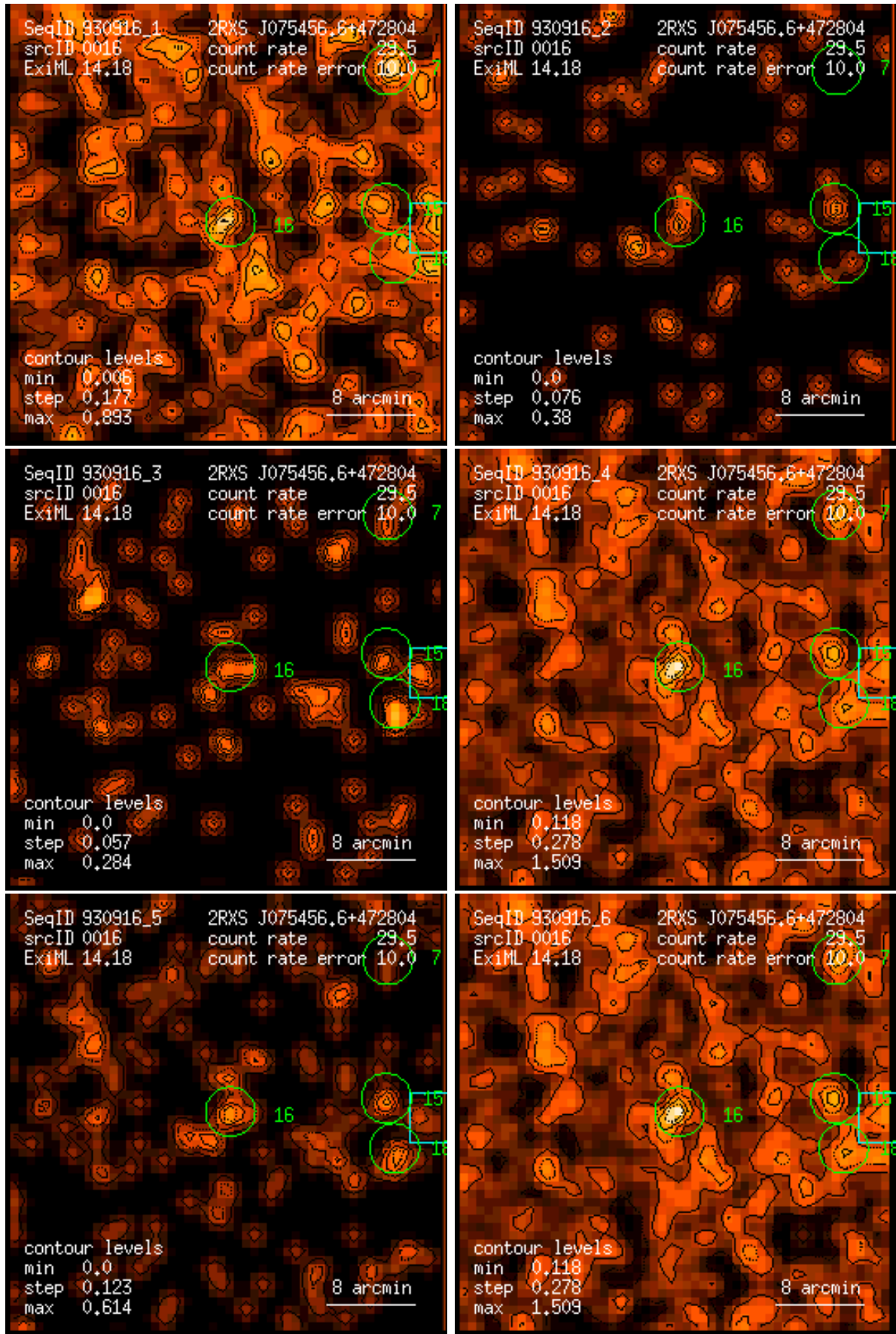
Figure 16: RASS 930916: detection 0016: band rate images, Gaussian filter: (1) PSPC channels 11 – 41, (2) 52 – 90, (3) 91 – 201, (4) 11 – 235, (5) 52 – 201, (6) 11 – 201. Broad band rates in counts/ks. Band rate contour levels in counts/ks/arcmin 2 .
