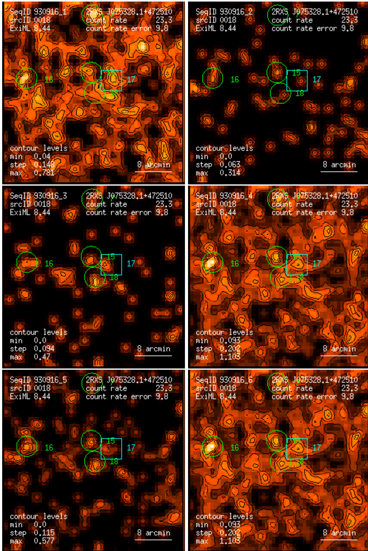
Figure 18: RASS 930916: detection 0018: band rate images, Gaussian filter: (1) PSPC channels 11 – 41, (2) 52 – 90, (3) 91 – 201, (4) 11 – 235, (5) 52 – 201, (6) 11 – 201. Broad band rates in counts/ks. Band rate contour levels in counts/ks/arcmin 2 .
