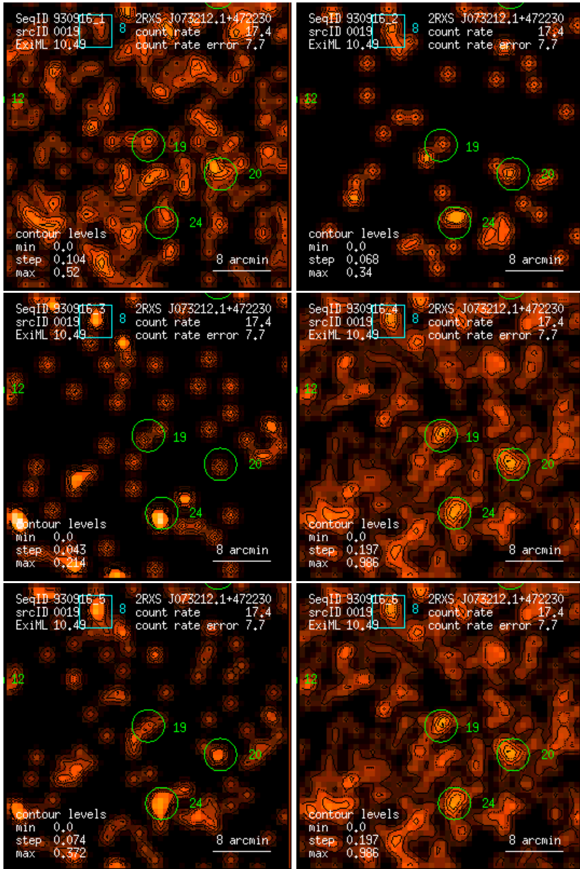
Figure 19: RASS 930916: detection 0019: band rate images, Gaussian filter: (1) PSPC channels 11 – 41, (2) 52 – 90, (3) 91 – 201, (4) 11 – 235, (5) 52 – 201, (6) 11 – 201. Broad band rates in counts/ks. Band rate contour levels in counts/ks/arcmin 2 .
