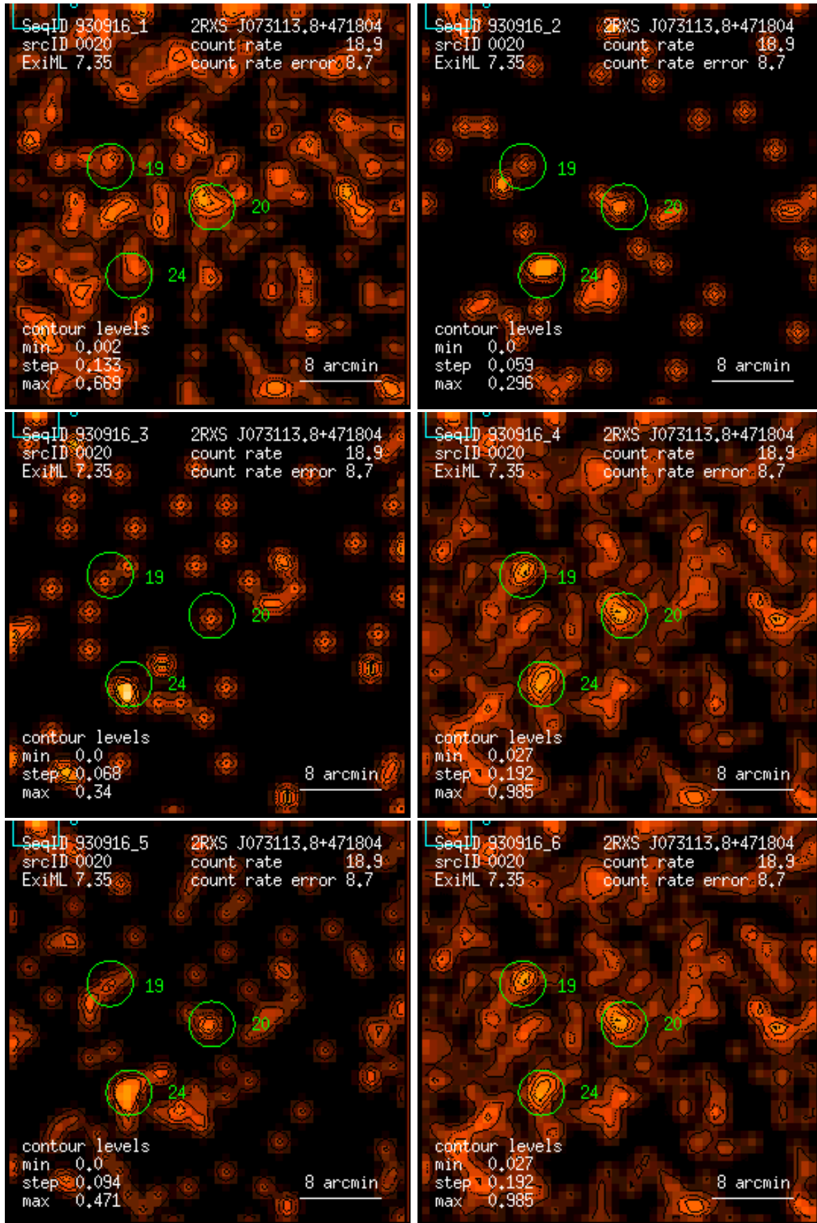
Figure 20: RASS 930916: detection 0020: band rate images, Gaussian filter: (1) PSPC channels 11 – 41, (2) 52 – 90, (3) 91 – 201, (4) 11 – 235, (5) 52 – 201, (6) 11 – 201. Broad band rates in counts/ks. Band rate contour levels in counts/ks/arcmin 2 .
