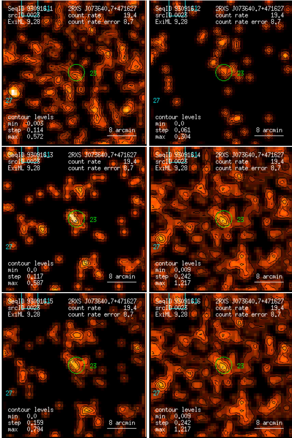
Figure 23: RASS 930916: detection 0023: band rate images, Gaussian filter: (1) PSPC channels 11 – 41, (2) 52 – 90, (3) 91 – 201, (4) 11 – 235, (5) 52 – 201, (6) 11 – 201. Broad band rates in counts/ks. Band rate contour levels in counts/ks/arcmin 2 .
