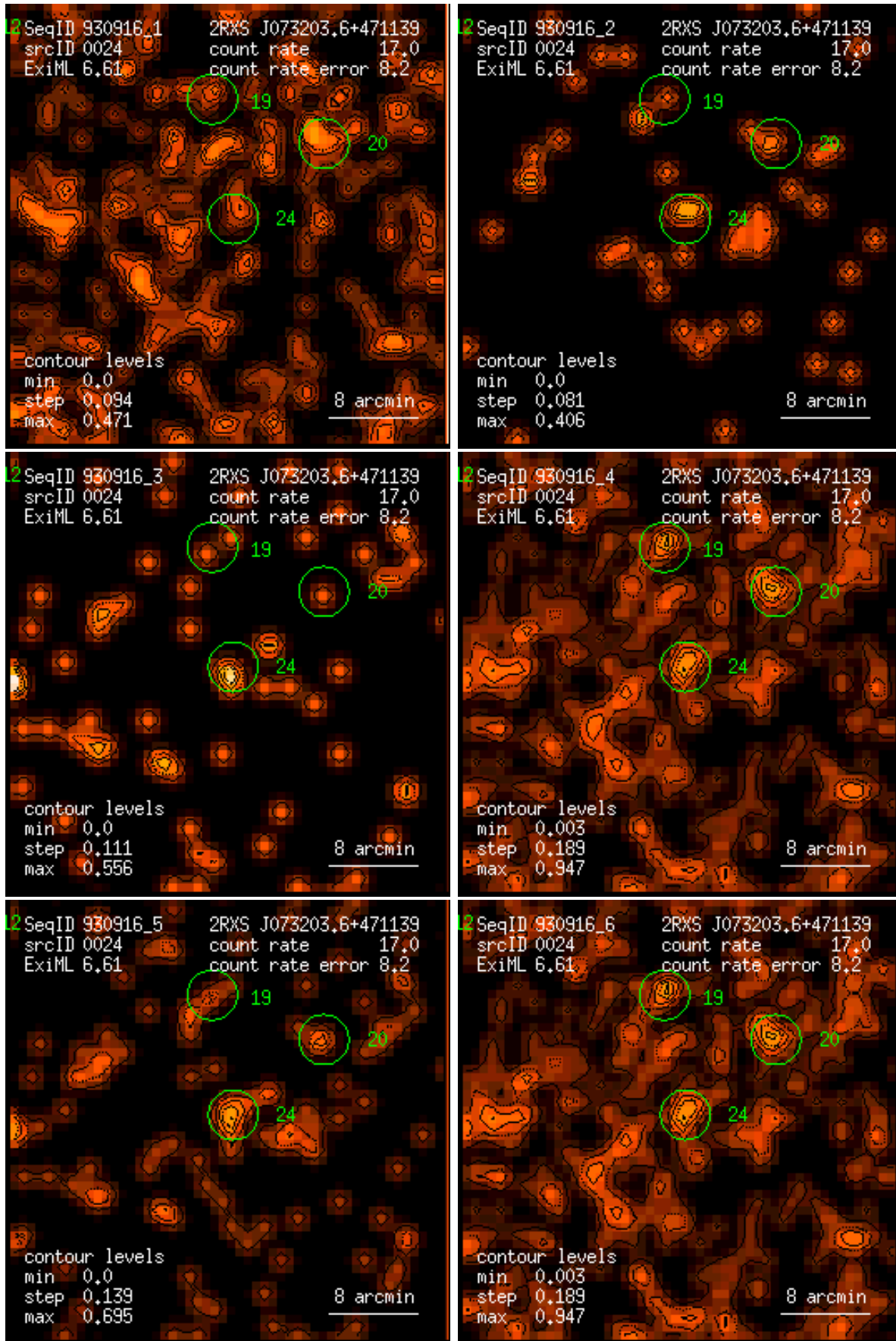
Figure 24: RASS 930916: detection 0024: band rate images, Gaussian filter: (1) PSPC channels 11 – 41, (2) 52 – 90, (3) 91 – 201, (4) 11 – 235, (5) 52 – 201, (6) 11 – 201. Broad band rates in counts/ks. Band rate contour levels in counts/ks/arcmin 2 .
