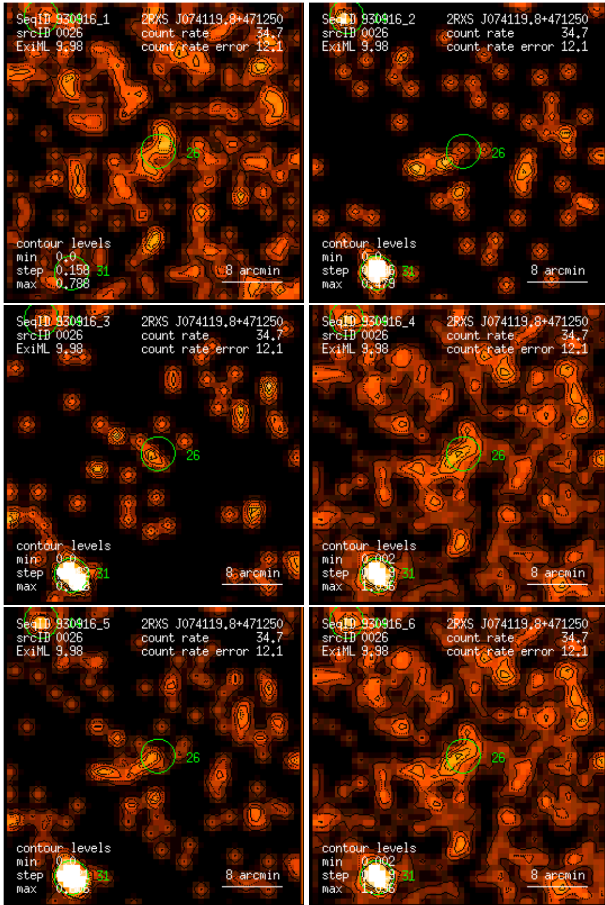
Figure 26: RASS 930916: detection 0026: band rate images, Gaussian filter: (1) PSPC channels 11 – 41, (2) 52 – 90, (3) 91 – 201, (4) 11 – 235, (5) 52 – 201, (6) 11 – 201. Broad band rates in counts/ks. Band rate contour levels in counts/ks/arcmin 2 .
