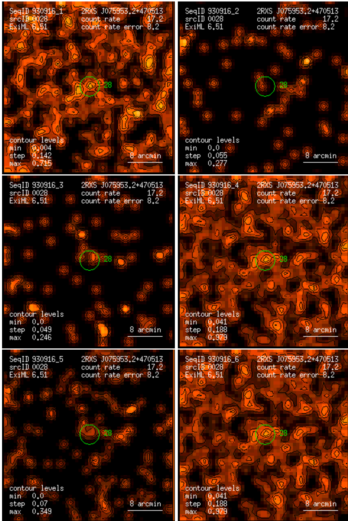
Figure 28: RASS 930916: detection 0028: band rate images, Gaussian filter: (1) PSPC channels 11 – 41, (2) 52 – 90, (3) 91 – 201, (4) 11 – 235, (5) 52 – 201, (6) 11 – 201. Broad band rates in counts/ks. Band rate contour levels in counts/ks/arcmin 2 .
