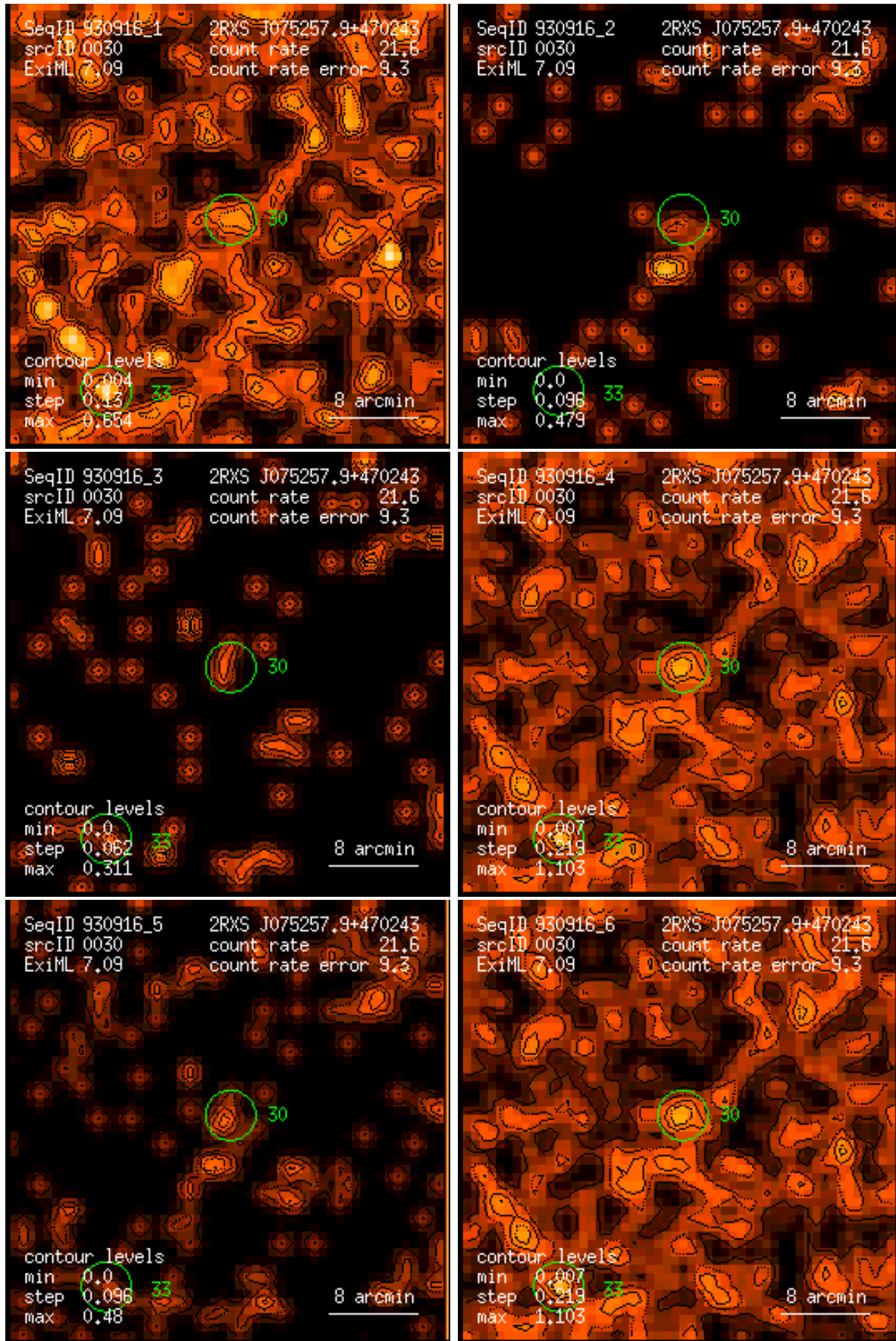
Figure 30: RASS 930916: detection 0030: band rate images, Gaussian filter: (1) PSPC channels 11 – 41, (2) 52 – 90, (3) 91 – 201, (4) 11 – 235, (5) 52 – 201, (6) 11 – 201. Broad band rates in counts/ks. Band rate contour levels in counts/ks/arcmin 2 .
