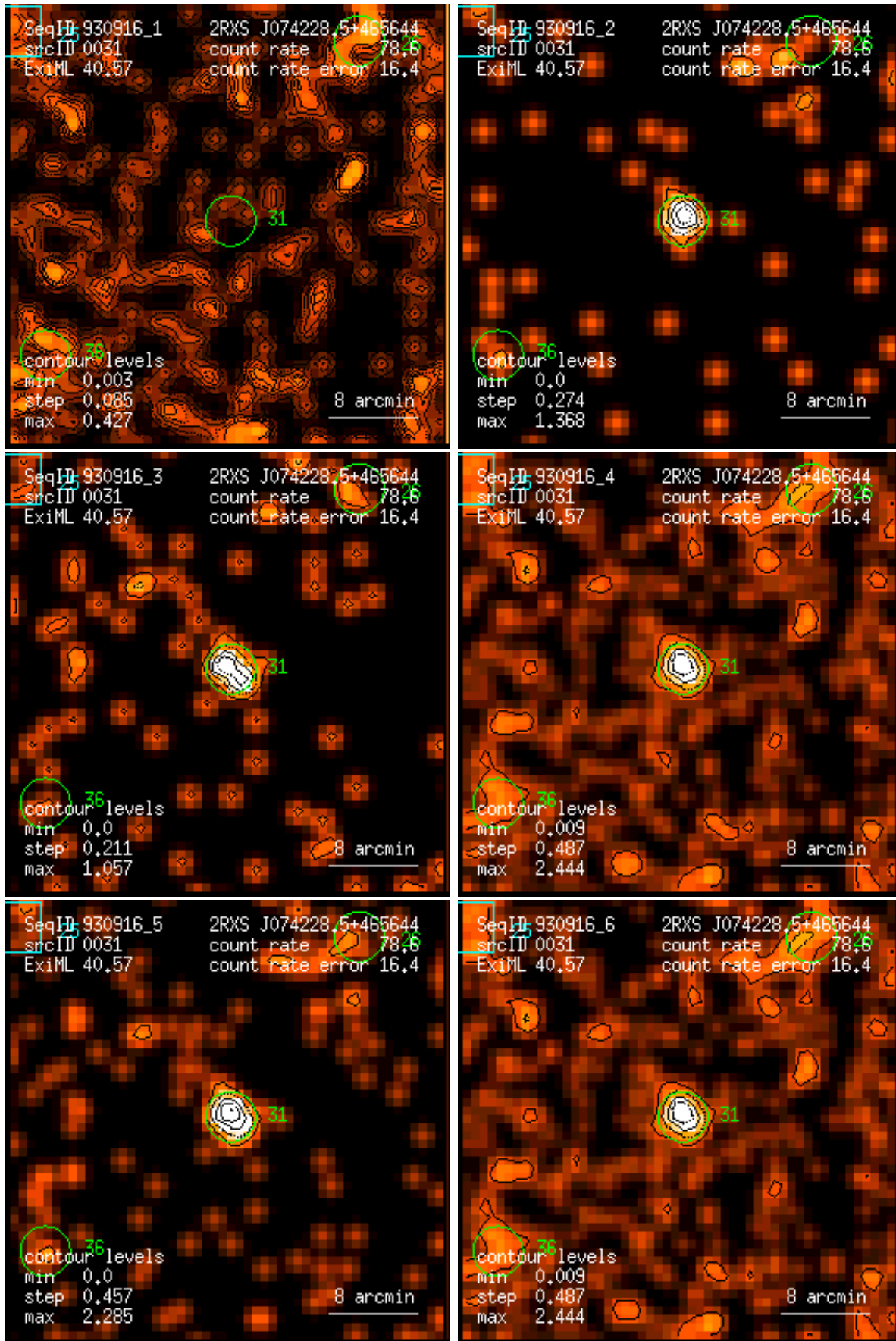
Figure 31: RASS 930916: detection 0031: band rate images, Gaussian filter: (1) PSPC channels 11 – 41, (2) 52 – 90, (3) 91 – 201, (4) 11 – 235, (5) 52 – 201, (6) 11 – 201. Broad band rates in counts/ks. Band rate contour levels in counts/ks/arcmin 2 .
