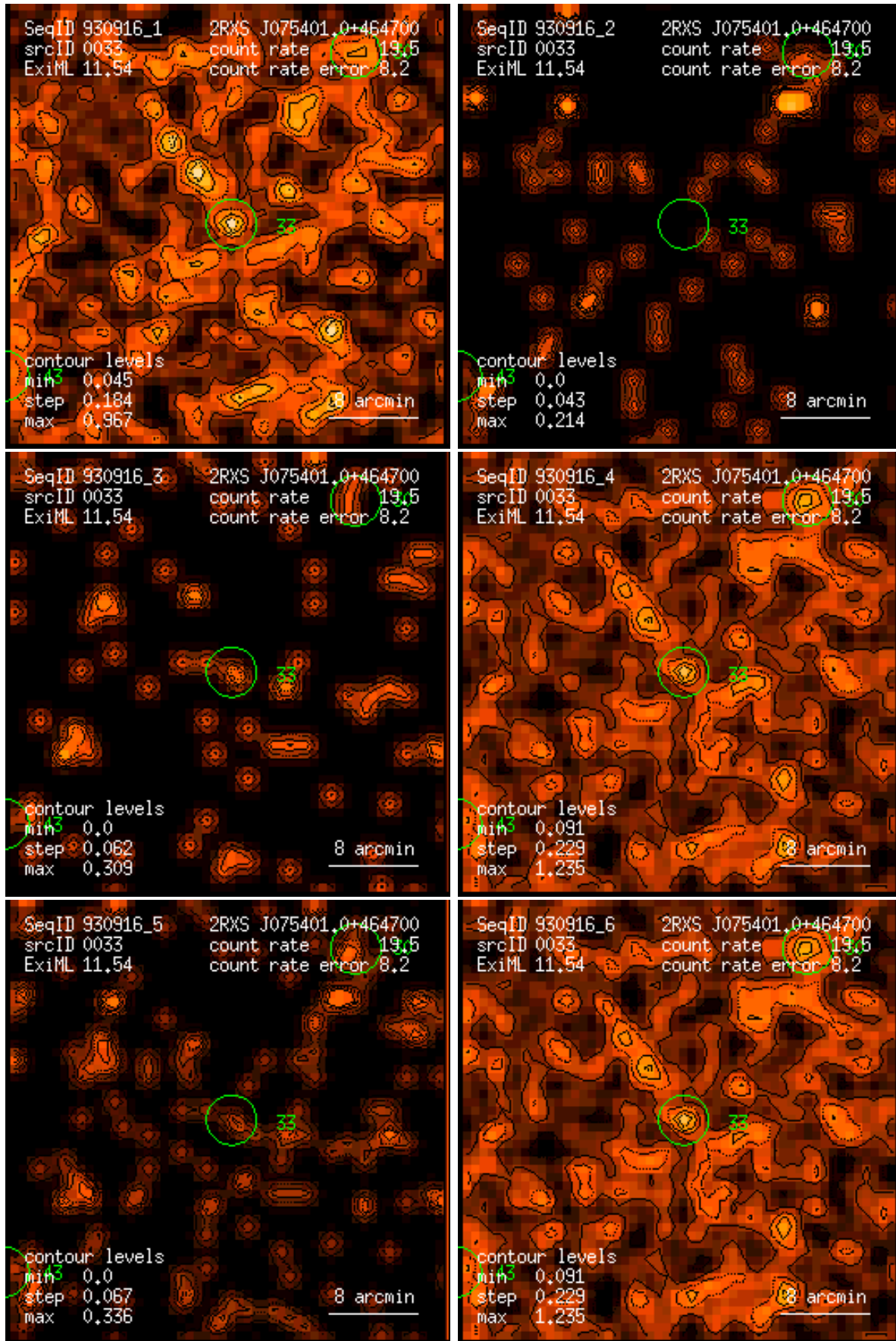
Figure 33: RASS 930916: detection 0033: band rate images, Gaussian filter: (1) PSPC channels 11 – 41, (2) 52 – 90, (3) 91 – 201, (4) 11 – 235, (5) 52 – 201, (6) 11 – 201. Broad band rates in counts/ks. Band rate contour levels in counts/ks/arcmin 2 .
