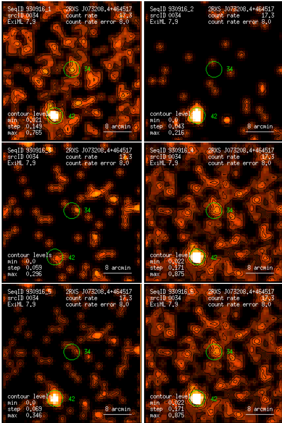
Figure 34: RASS 930916: detection 0034: band rate images, Gaussian filter: (1) PSPC channels 11 – 41, (2) 52 – 90, (3) 91 – 201, (4) 11 – 235, (5) 52 – 201, (6) 11 – 201. Broad band rates in counts/ks. Band rate contour levels in counts/ks/arcmin 2 .
