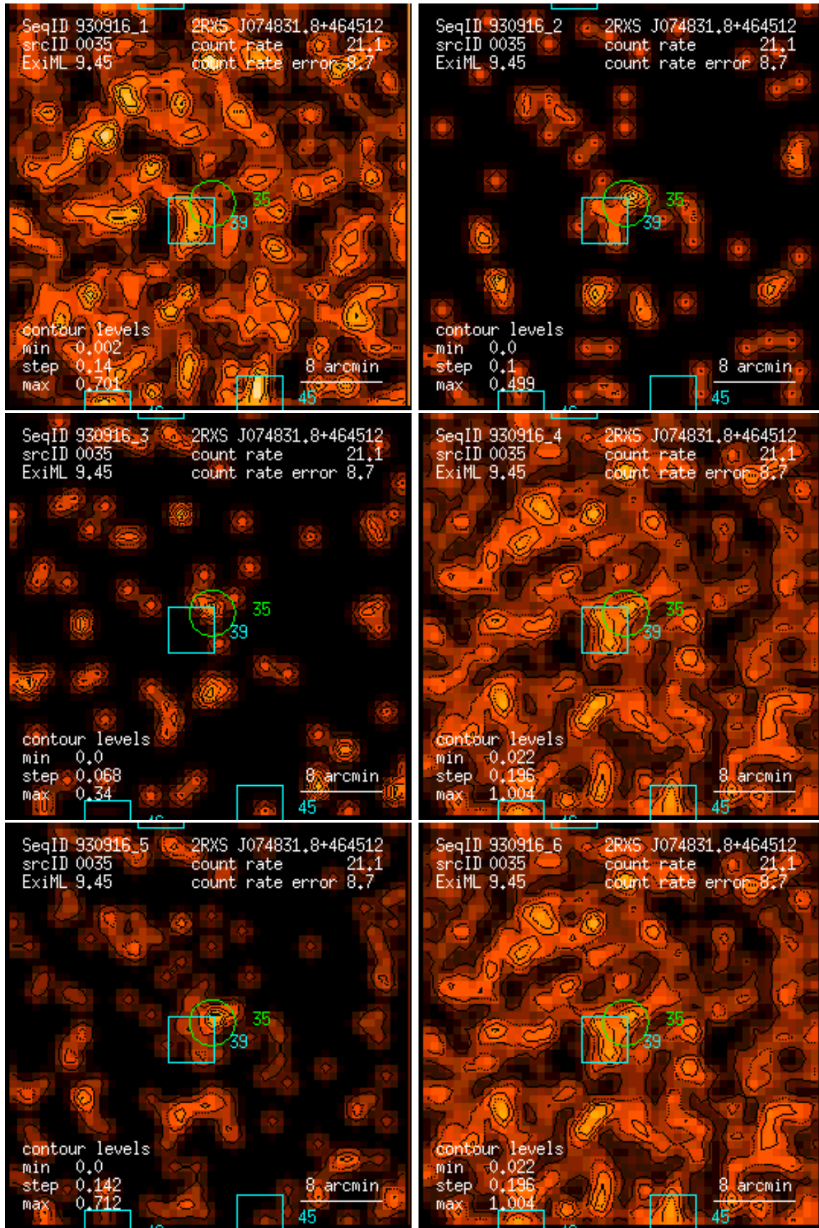
Figure 35: RASS 930916: detection 0035: band rate images, Gaussian filter: (1) PSPC channels 11 – 41, (2) 52 – 90, (3) 91 – 201, (4) 11 – 235, (5) 52 – 201, (6) 11 – 201. Broad band rates in counts/ks. Band rate contour levels in counts/ks/arcmin 2 .
