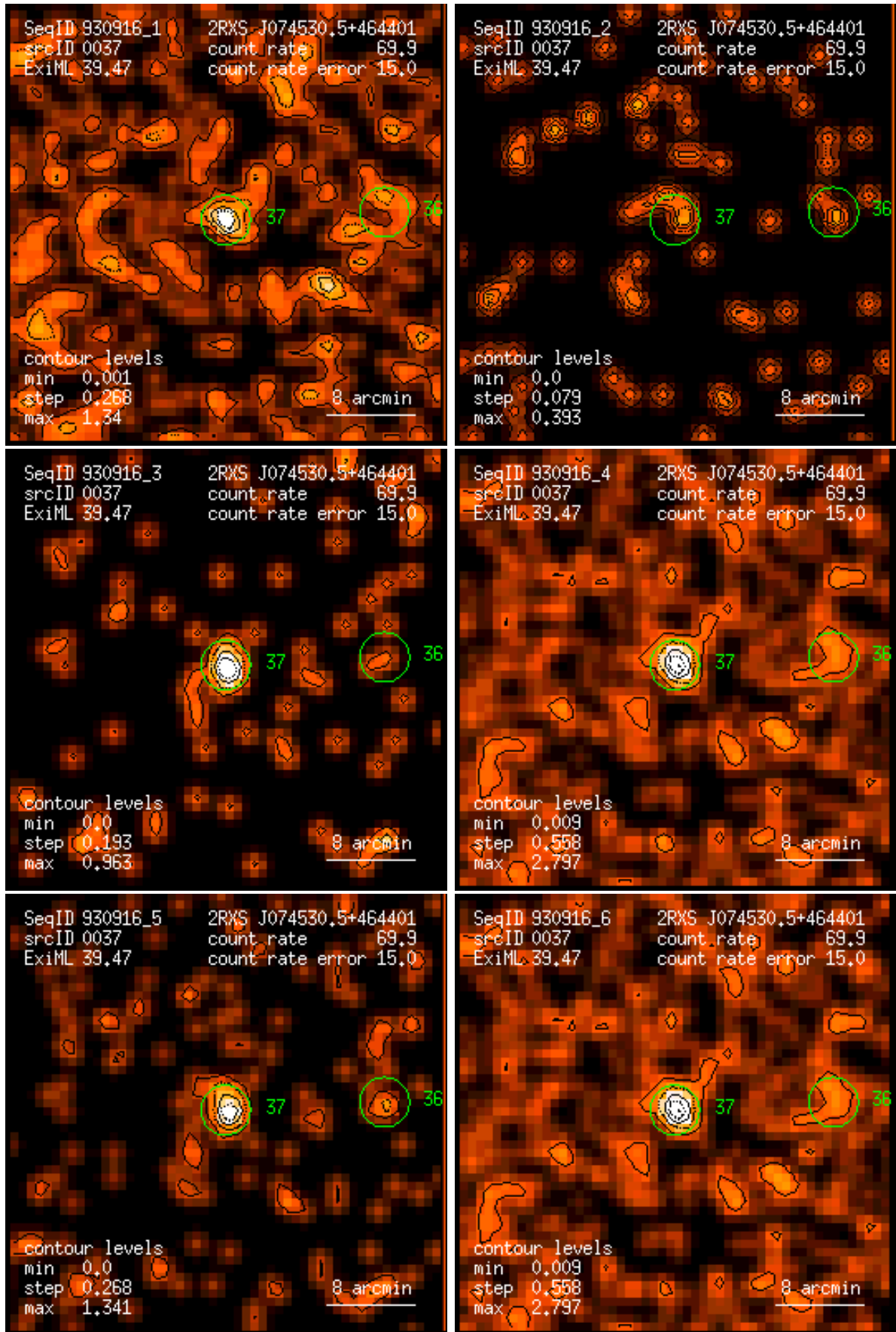
Figure 37: RASS 930916: detection 0037: band rate images, Gaussian filter: (1) PSPC channels 11 – 41, (2) 52 – 90, (3) 91 – 201, (4) 11 – 235, (5) 52 – 201, (6) 11 – 201. Broad band rates in counts/ks. Band rate contour levels in counts/ks/arcmin 2 .
