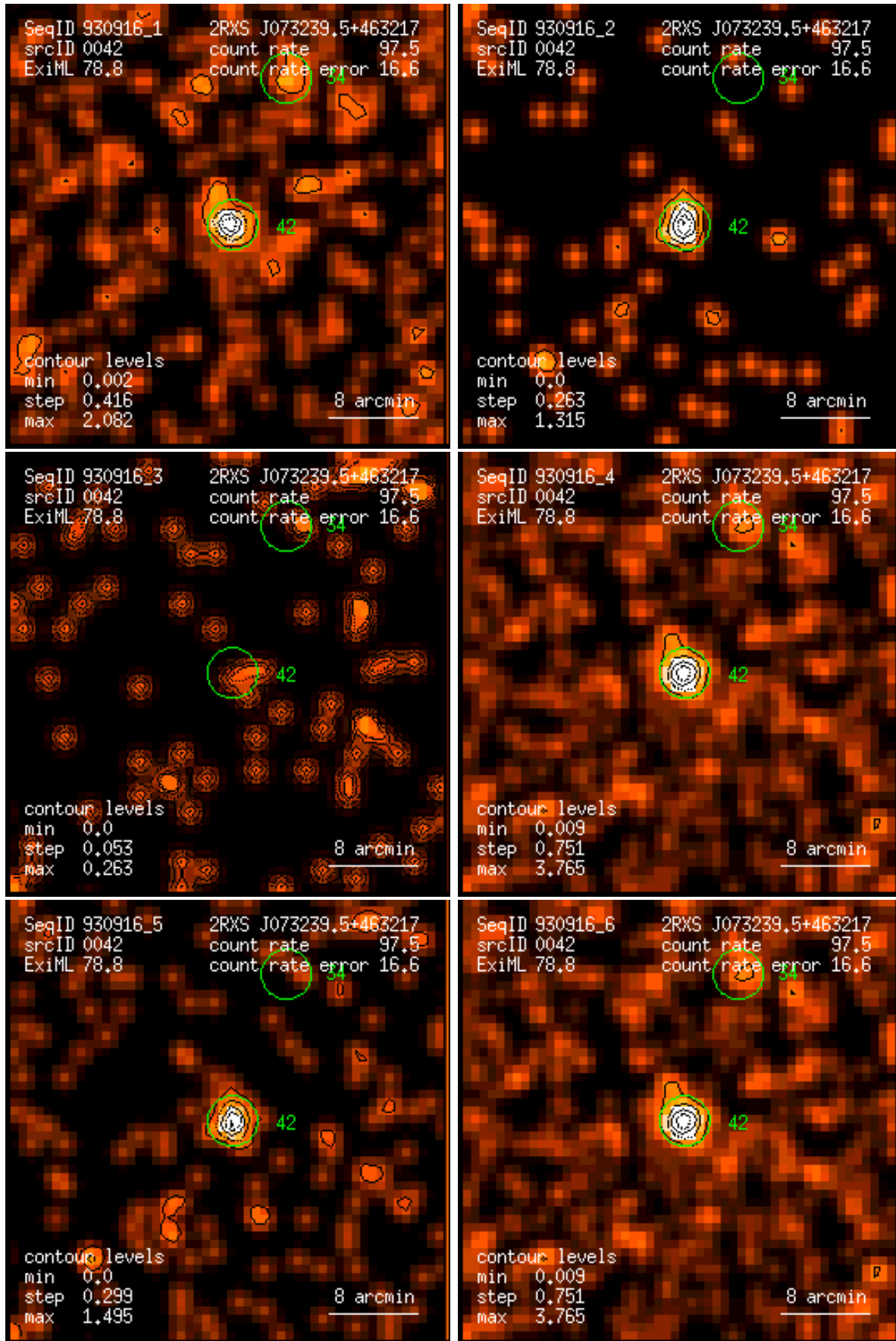
Figure 42: RASS 930916: detection 0042: band rate images, Gaussian filter: (1) PSPC channels 11 – 41, (2) 52 – 90, (3) 91 – 201, (4) 11 – 235, (5) 52 – 201, (6) 11 – 201. Broad band rates in counts/ks. Band rate contour levels in counts/ks/arcmin 2 .
