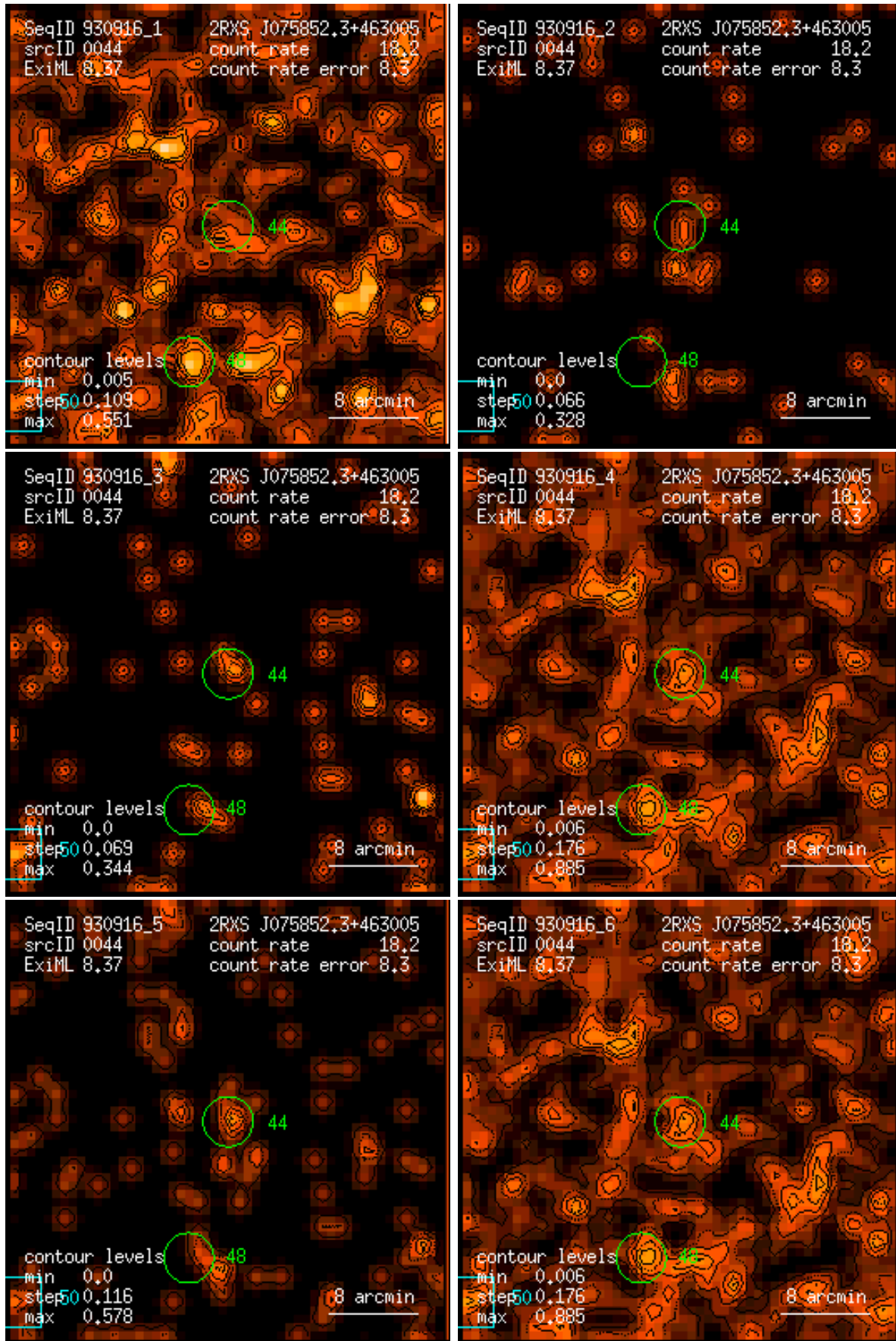
Figure 44: RASS 930916: detection 0044: band rate images, Gaussian filter: (1) PSPC channels 11 – 41, (2) 52 – 90, (3) 91 – 201, (4) 11 – 235, (5) 52 – 201, (6) 11 – 201. Broad band rates in counts/ks. Band rate contour levels in counts/ks/arcmin 2 .
