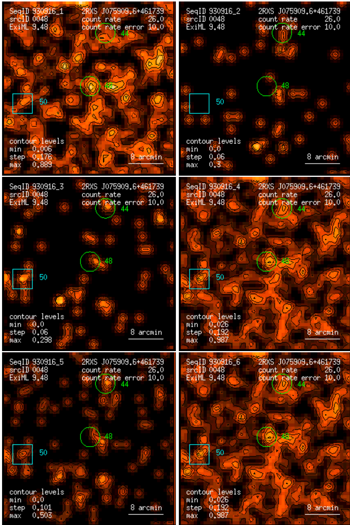
Figure 48: RASS 930916: detection 0048: band rate images, Gaussian filter: (1) PSPC channels 11 – 41, (2) 52 – 90, (3) 91 – 201, (4) 11 – 235, (5) 52 – 201, (6) 11 – 201. Broad band rates in counts/ks. Band rate contour levels in counts/ks/arcmin 2 .
