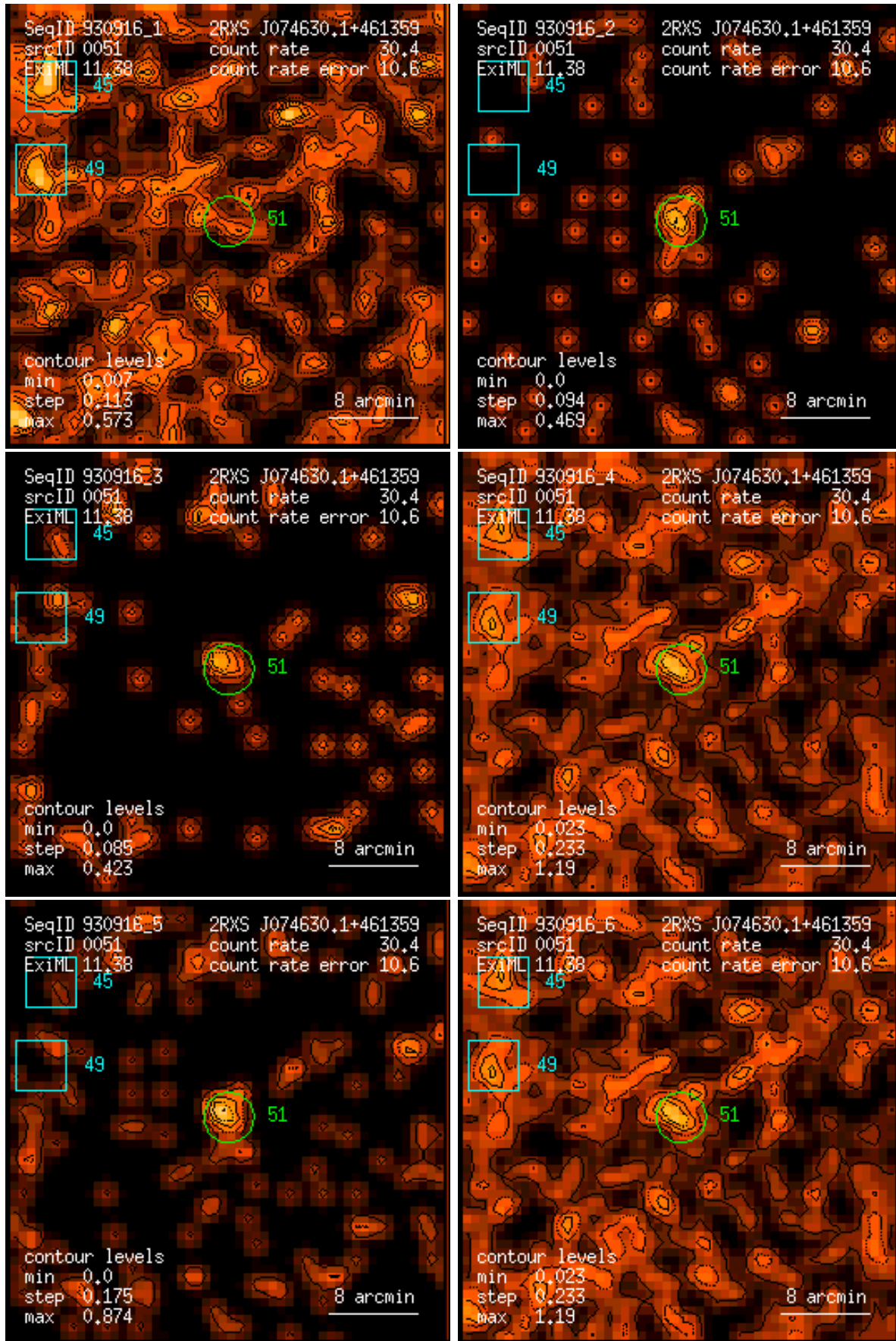
Figure 51: RASS 930916: detection 0051: band rate images, Gaussian filter: (1) PSPC channels 11 – 41, (2) 52 – 90, (3) 91 – 201, (4) 11 – 235, (5) 52 – 201, (6) 11 – 201. Broad band rates in counts/ks. Band rate contour levels in counts/ks/arcmin 2 .
