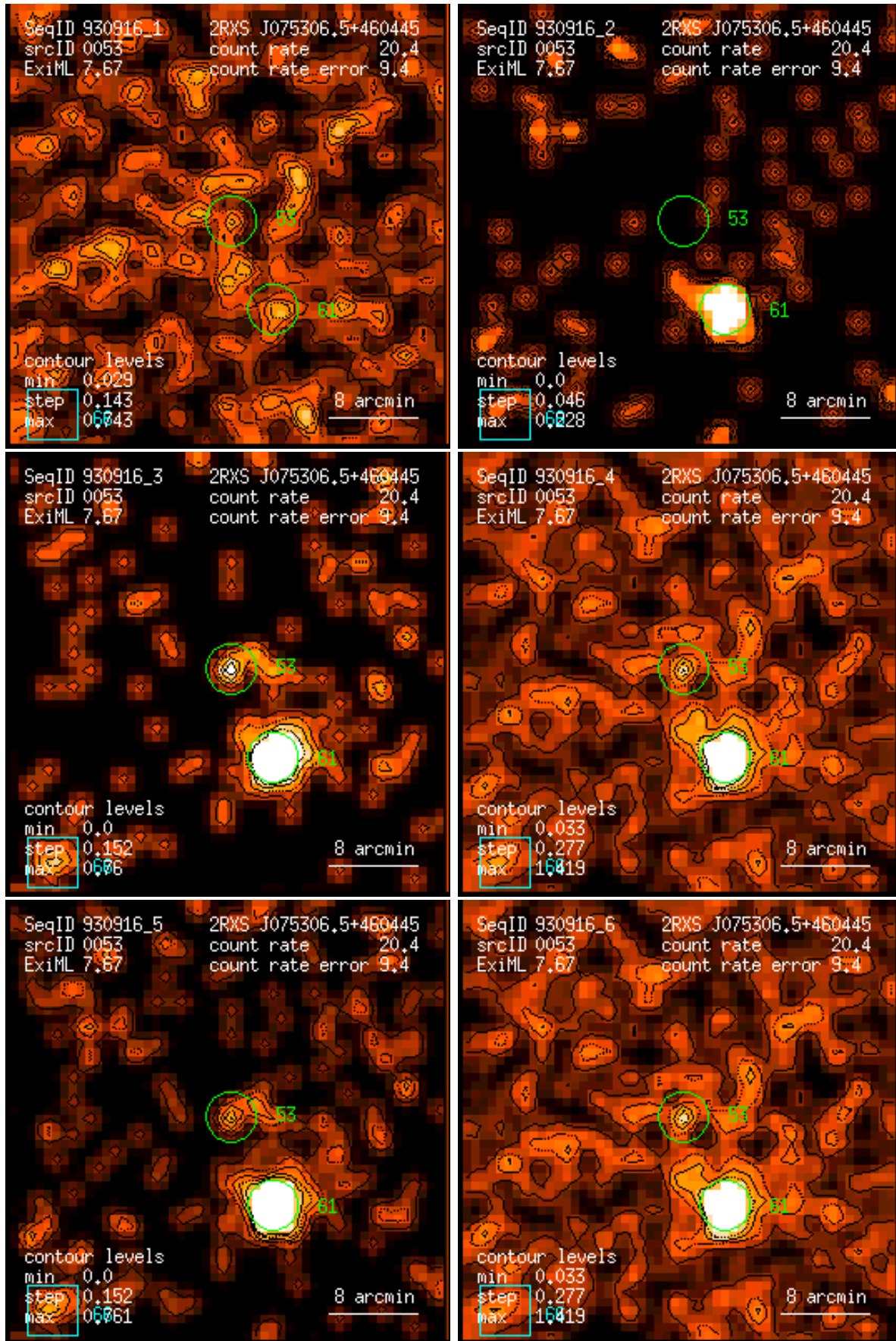
Figure 53: RASS 930916: detection 0053: band rate images, Gaussian filter: (1) PSPC channels 11 – 41, (2) 52 – 90, (3) 91 – 201, (4) 11 – 235, (5) 52 – 201, (6) 11 – 201. Broad band rates in counts/ks. Band rate contour levels in counts/ks/arcmin 2 .
