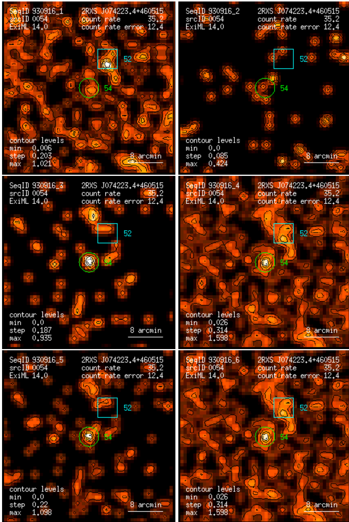
Figure 54: RASS 930916: detection 0054: band rate images, Gaussian filter: (1) PSPC channels 11 – 41, (2) 52 – 90, (3) 91 – 201, (4) 11 – 235, (5) 52 – 201, (6) 11 – 201. Broad band rates in counts/ks. Band rate contour levels in counts/ks/arcmin 2 .
